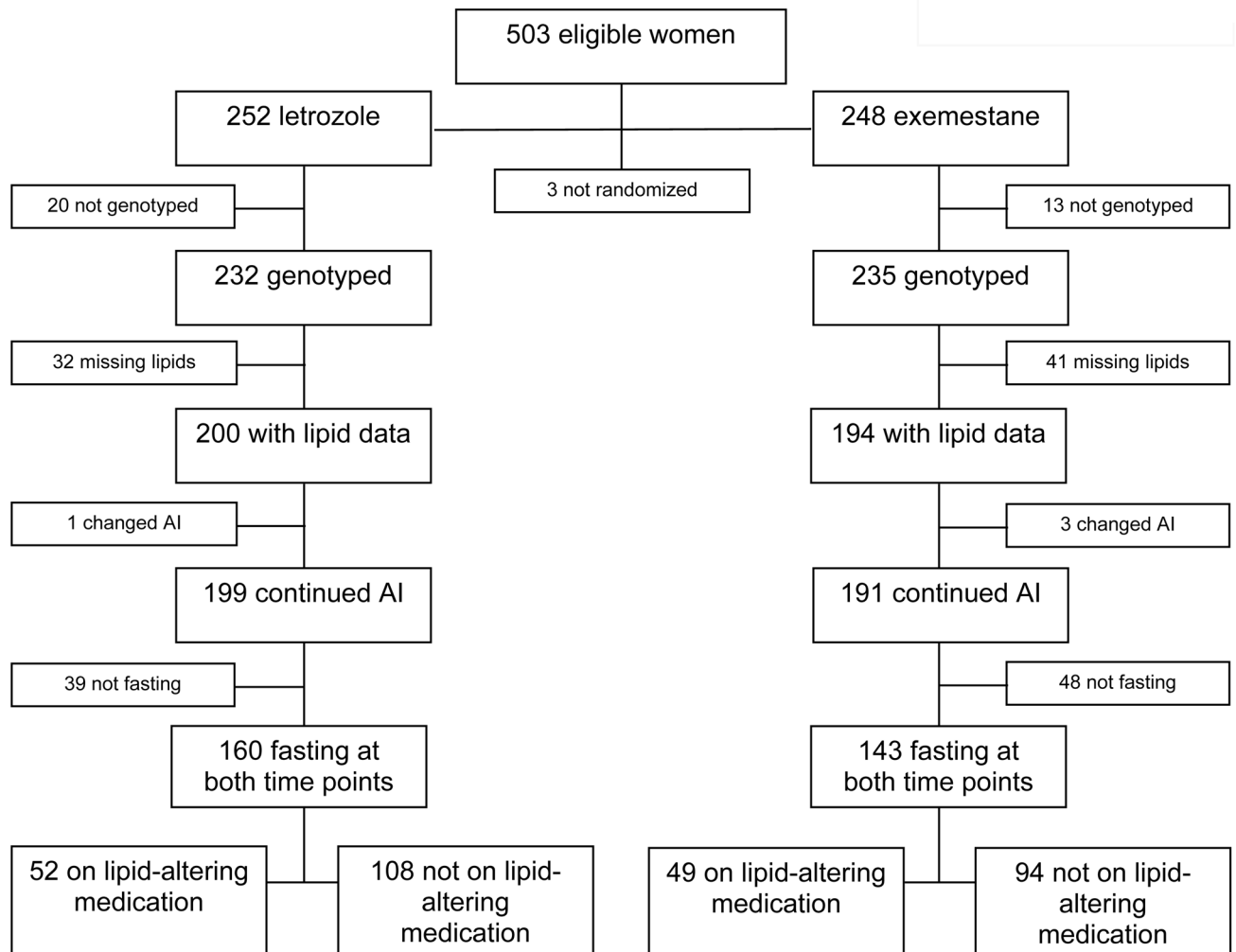
Figure 1. Consort diagram.
