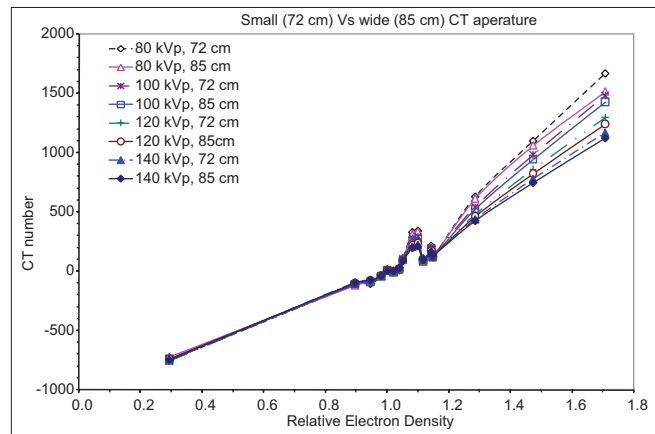
Figure 3: Comparison of computed tomography number for Philips PQ5000 with different apertures (72 cm and 85 cm). There is a very little difference in computed tomography number between two scanners
