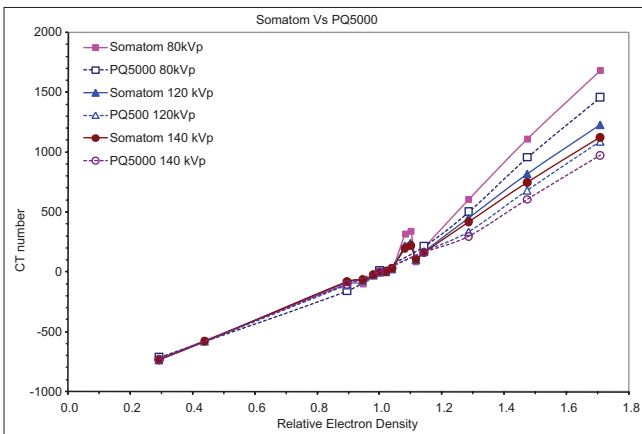
Figure 2: Comparison of computed tomography number from two different manufacturers (Philips and Siemens) with same scan aperture and reconstructed field of view. Note significant changes in computed tomography number for bone with two scanners
