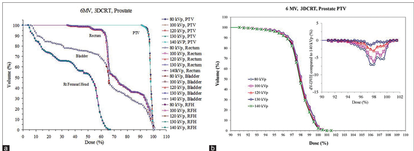
Figure 5: (a) Comparison of dose-volume histogram for a prostate three-dimensional conformal radiation therapy with various electron densities associated with tube voltages (80–140 kVp) and (b) magnified view of dose-volume histogram for planning target volume only. Also note the plot of dV-dose-volume histogram in inset providing useful information where dose-volume histogram cannot be easily differentiated
