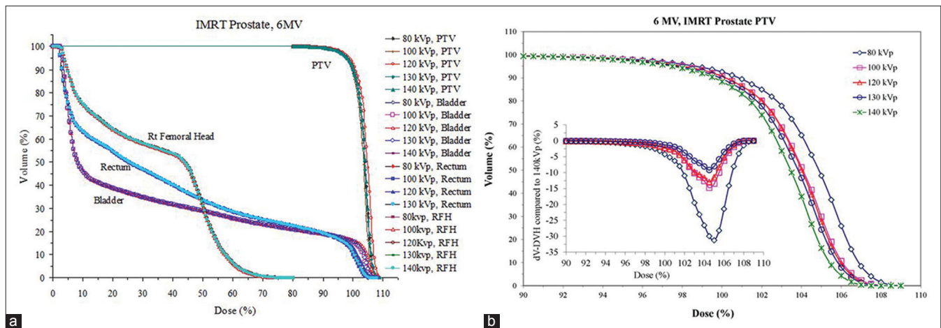
Figure 6: (a) Comparison of dose-volume histogram for a prostate intensity-modulated radiation therapy with various electron densities associated with tube voltages (80–140 kVp) and (b) magnified view of dose-volume histogram for planning target volume only. Also note the plot of dV-dose-volume histogram in inset providing useful information where dose-volume histograms cannot be easily differentiated
