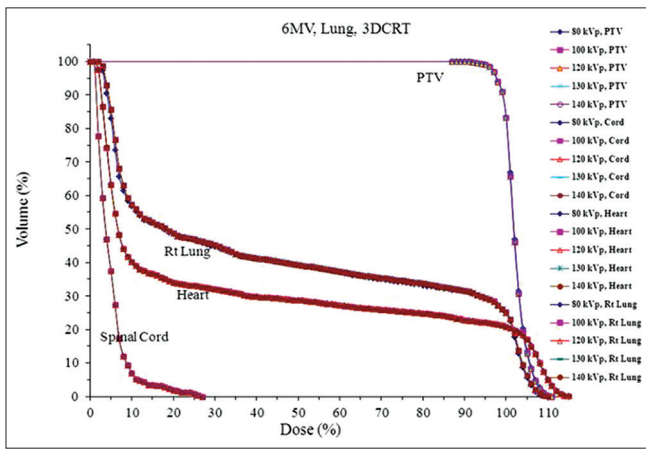
Figure 4: Dose-volume histograms of planning target volume, spinal cord, heart and lung of a tumor lesion centrally located in the right lung calculated using computed tomography number to electron density calibrations of different tube voltages (80–140 kVp)
