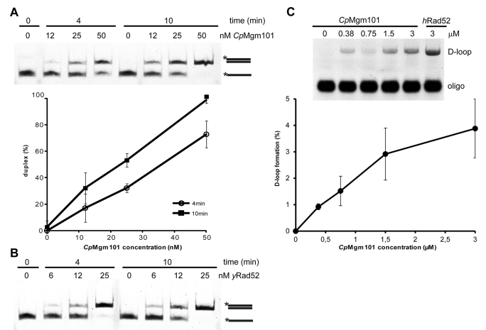
Figure 4. The single-strand annealing and strand invasion activities of CpMgm101 protein. The single-strand annealing activities of (A) CpMgm101 and (B) yRad52 . The reactions were carried out using 3 nM of labeled Oligo1 and 8 nM of unlabeled Oligo2 with increasing concentrations of protein (see 'Materials and Methods' section). The plot shows the averaged results of three independent experiments. (C) The strand invasion activity of CpMgm101 . The reactions were carried out on pBluescript replicative form I using a protein-Oligo8 complex that had been previously formed by incubating 40 nM of fluorescently labeled 90-base Oligo8 with increasing concentrations (0.38, 0.75, 1.5, 3 μM) of CpMgm101 (at 30°C) or 3 μM of hRad52 (at 37°C) proteins for 10 min (see 'Materials and Methods' section).
