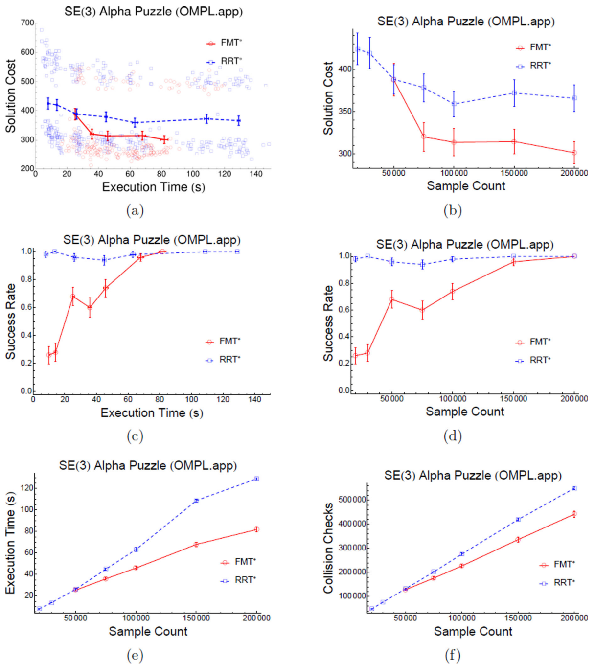
Figure 13. Simulation results for a Alpha puzzle.
