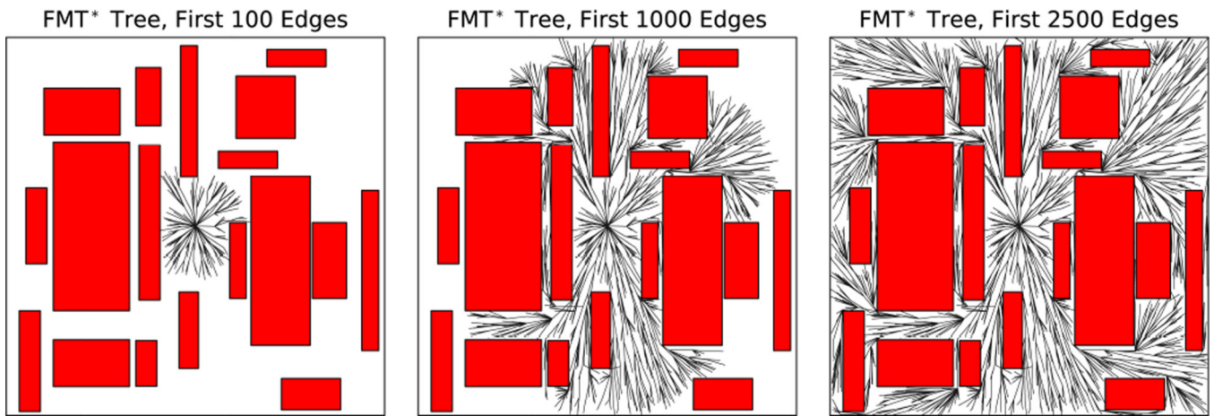
Figure 1. The FMT* algorithm generates a tree by moving steadily outward in cost-to-arrive space. This figure portrays the growth of the tree in a 2D environment with 2,500 samples (only edges are shown).
