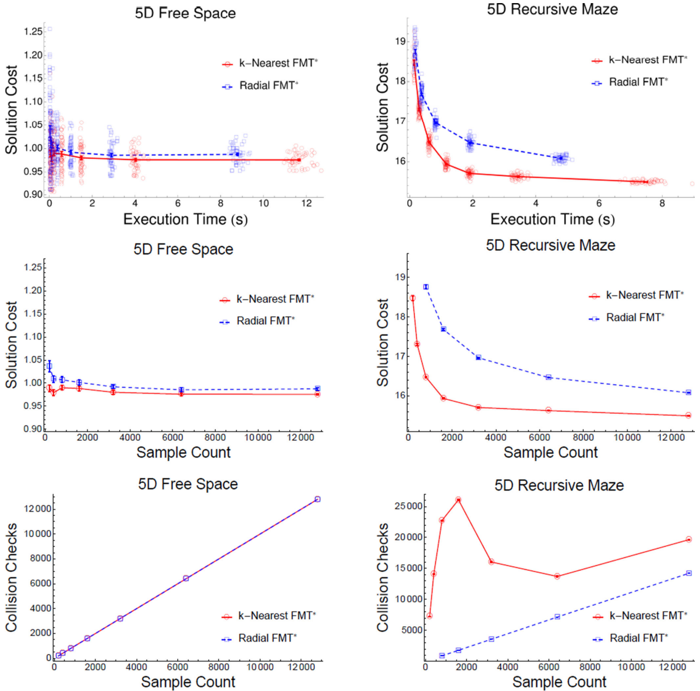
Figure 14. Comparison between radial-FMT* and k -nearest FMT*.
