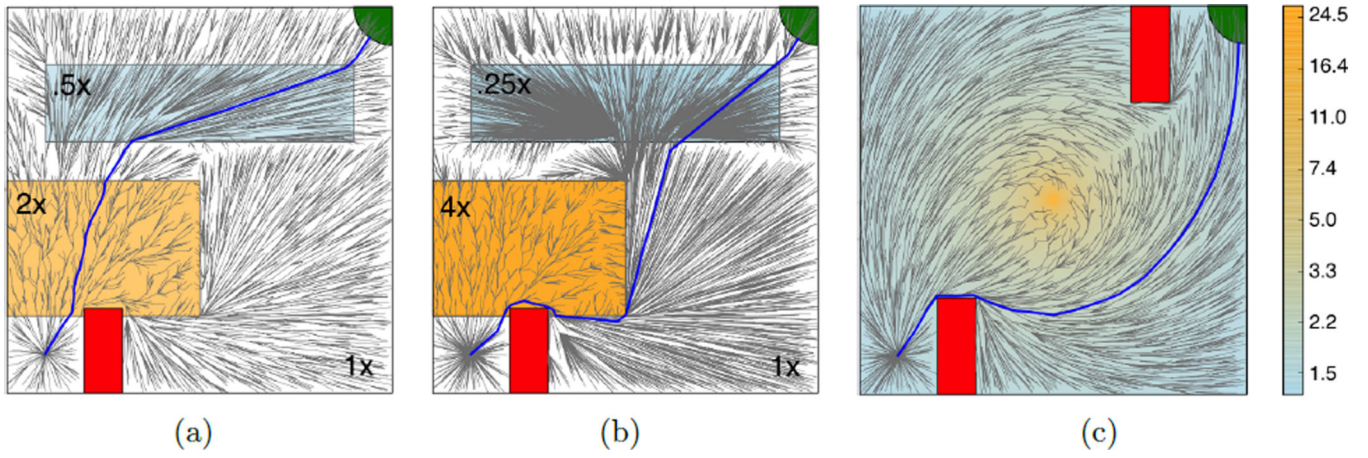
Figure 17. Planning with general costs.
