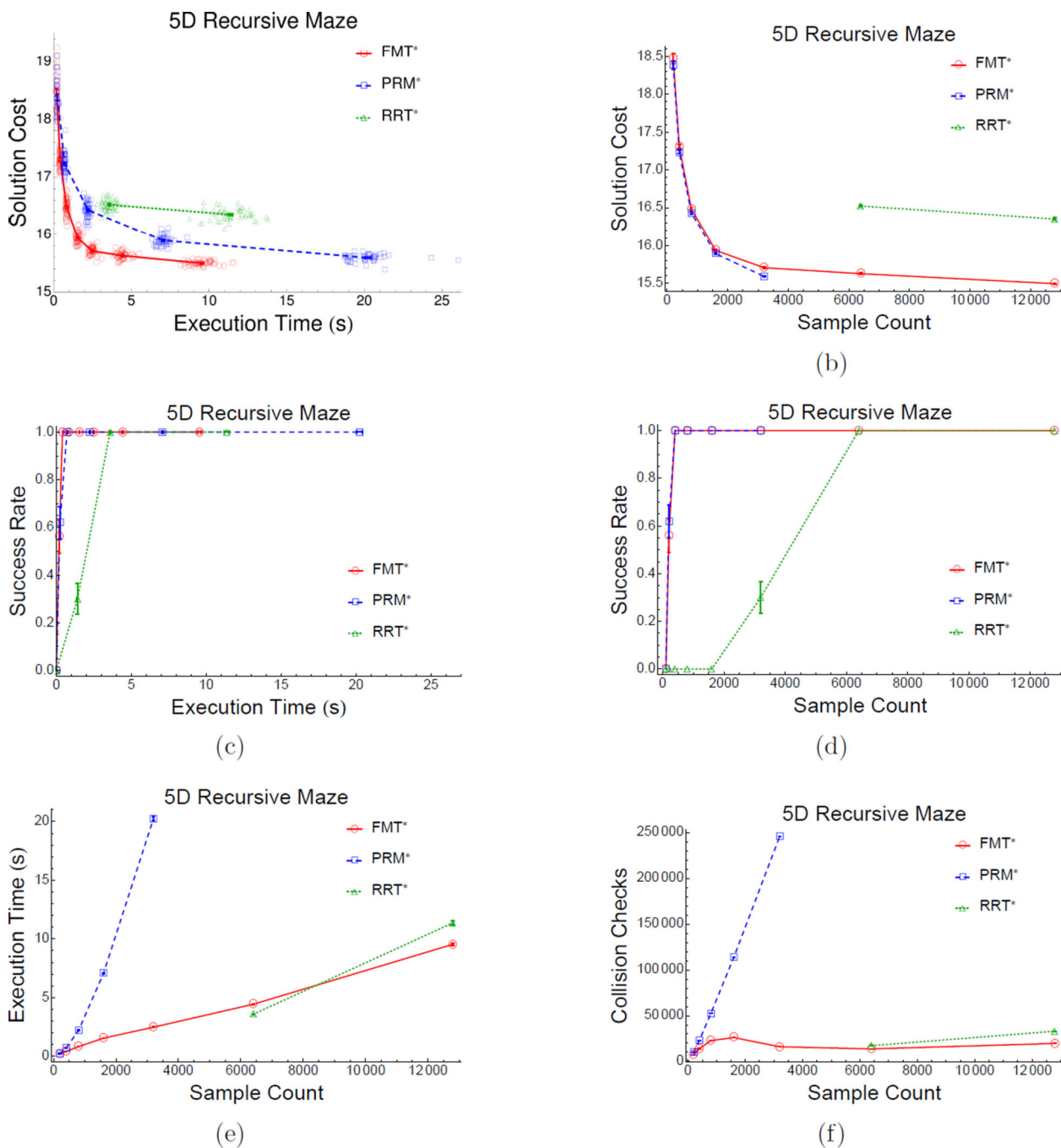
Figure 11. Simulation results for a recursive maze environment in 5D.
