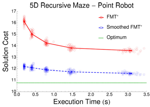
Figure 16. Simulation results for a maze configuration in 5D space.
