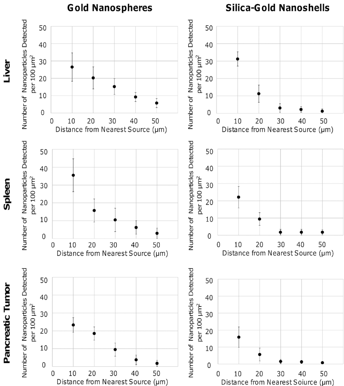
Fig. 5. Penetration of PC-coated gold NPs in liver, spleen, and pancreatic tumor tissues [70]. Particles were visualized using hyperspectral imaging, and their distances measured from nearest source points. In the liver and pancreatic tumor, gold nanospheres had linear diffusion, while in the spleen it was an exponential decline. Silica gold nanoshells had an exponential decline for all tissue types, suggesting limited diffusivity. Their extravasation was highest in the liver, while for gold nanospheres it was highest in the spleen. All error
