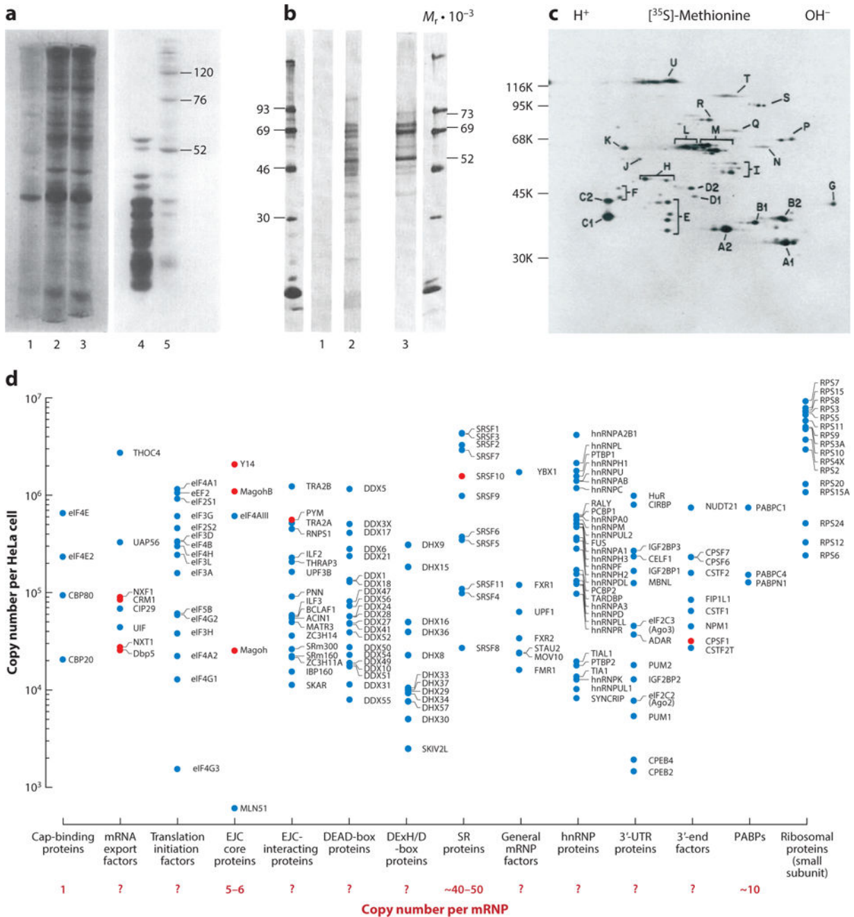
Figure 1. Identification and relative abundance of mRNP components. (a) Oligo-dT-cellulose-selected nuclear hnRNP or cytoplasmic mRNP proteins from [ 3 H]-uridine pulse-labeled HeLa cells. (Lanes 1–3) hnRNP proteins recovered from the unbound fraction (lane 1) or from elution with 25% formamide (lane 2) or with 50% formamide (lane 3). (Lanes 4–5) mRNP proteins in the unbound fraction (lane 4) (mainly ribosomal subunits) or eluted with 50% formamide (lane 5). Panel adapted with permission from plate I in Reference 3. (b) Proteins from oligo-dT-cellulose-selected polyribosomal RNPs from human KB cells labeled with [ 35 S]-methionine without (lane 1) or with (lane 2) short-wave UV irradiation. Oligo-dT-selected
