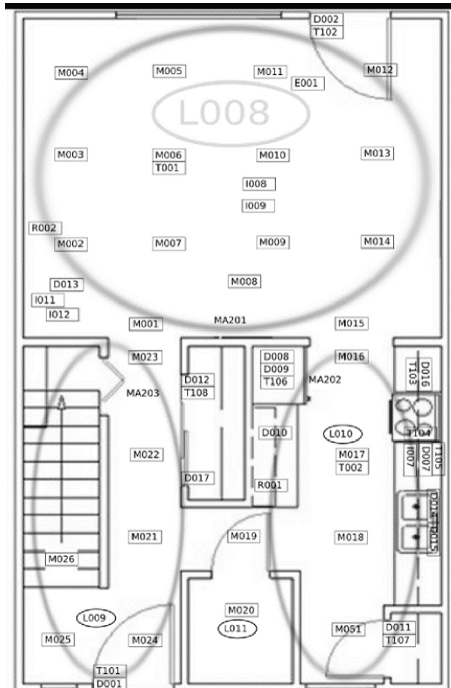
Fig. 1. The layout of the smart apartment and sensor placement. Sensor labels starting with “M” indicates motion sensors, “L” indicates light sensors, “D” indicates door sensors, “T” indicates temperature sensors, and “I” indicates item sensors.
