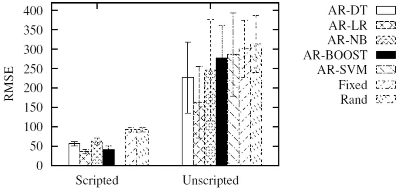
Fig. 6. RSME scores for supervised learning on the scripted and unscripted datasets. All of the AR techniques outperform the baseline techniques of Fixed and Random. Error bars represent the standard error of the mean.
