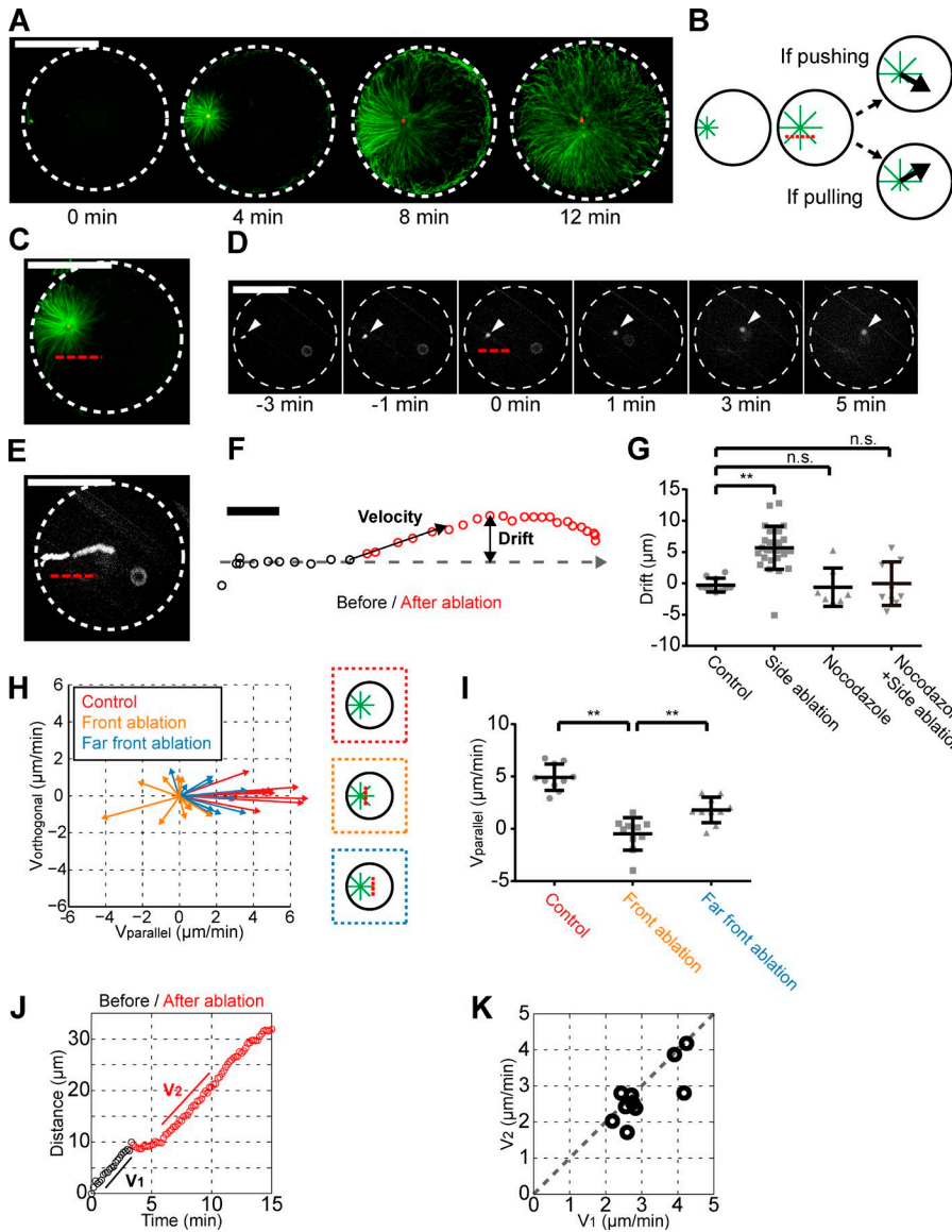
Figure 2. Aster centration is driven by MT-pulling forces in the cytoplasm. (A) Time-dependent immunostaining of centering MT asters (MT, green; DNA, red). The indicated time is taken in reference with sperm entry by accounting for a mean 3-min delay between sperm addition and entry. (B) Centering MT asters are ablated parallel to the centration trajectory. A drift in the trajectory toward (away from) the ablation line suggests that MTs are pushing (pulling). (C) In situ MT aster immunostaining performed immediately after laser ablation along the red broken line. (D and E) Time-lapse (D) and time projection (E) of a centering aster ablated as indicated. Time 0 is the time of ablation. White arrowhead, male pronucleus. (F) Definition of aster velocity and drift after ablation. (G) Aster drift in the indicated conditions ( n = 10 for control; n = 28 for side ablation; n = 7 for nocodazole; n = 10 for nocodazole + side ablation). Bar, 10 \mu\text{m} . (H) Aster velocity vectors after ablation at the indicated locations. (I) Aster speed along the centration path after ablation in the indicated conditions. (J) Distance–time plot of a front-ablated aster. (K) Aster velocity along the centration path after ablation ( V_2 ) as a function of the velocity before ( V_1 ). n.s., non-significant; **, P < 10^{-4} (Student's t test). Error bars represent SD. Bars, 50 \mu\text{m} .
