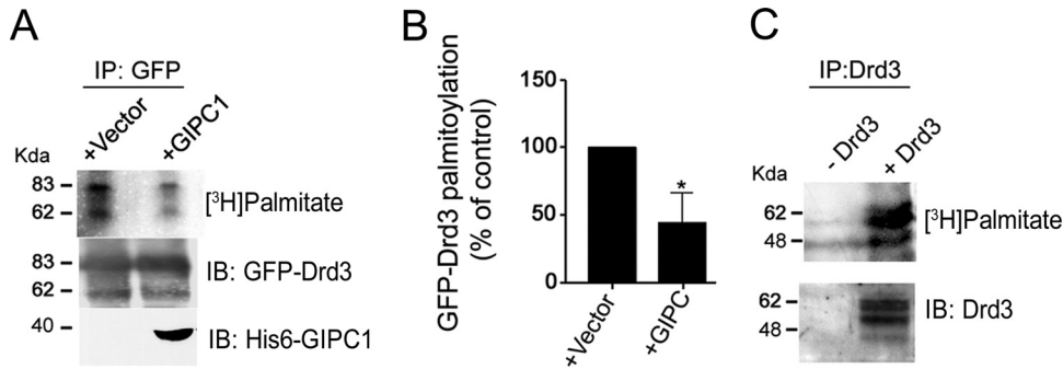
FIG 2 Drd3 palmitoylation and effect of GIPC1. (A) Incorporation of [ 3 H]palmitate in HEK293 cells transiently transfected with GFP-Drd3 and His6-GIPC1. Results of fluorography of immunopurified GFP-Drd3 using anti-GFP antibodies are shown. (B) Means ± SEM collected from 4 independent experiments (unpaired t test; P < 0.05). (C) Incorporation of [ 3 H]palmitate in Drd3 stably expressed in CHO cells. Fluorography results are shown for the radioactivity incorporated into Drd3 and for Western blotting of Drd3 protein immunopurified from cell lysates with specific antibodies against Drd3.
