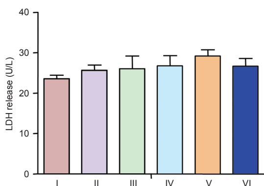
Figure 2 LDH release in cultured neurons treated with different concentrations of (Val 8 )GLP-1-Glu-PAL.
