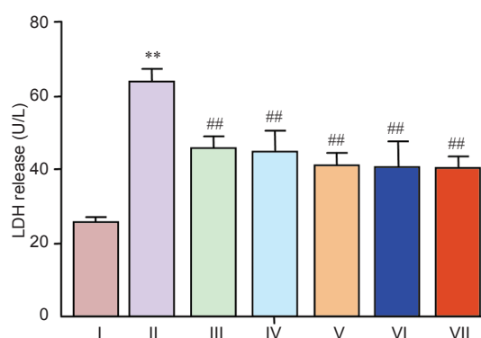
Figure 4 Rotenone-induced elevation of LDH release was inhibited by (Val 8 )GLP-1-Glu-PAL.
