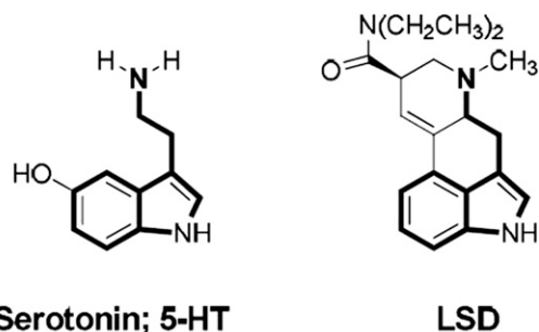
Fig. 1. Chemical structures of serotonin and LSD.
