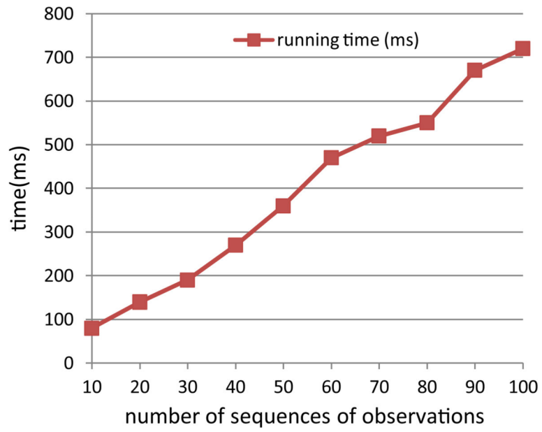
Fig. 21. Time of forward algorithm/Viterbi analysis with increasing # observation sequences
