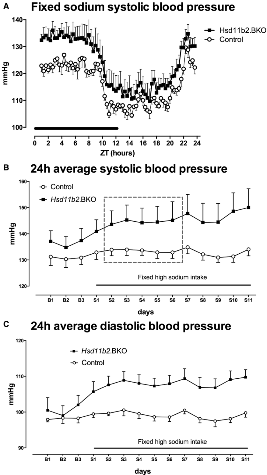
Figure 3. Radiotelemetry data from conscious unrestrained mice on fixed sodium intake. A , Systolic blood pressure measured every 20 minutes over a 24-hour period in Hsd11b2.BKO mice ( n=6 ; filled squares) and controls ( n=6 ; open circles). Data are group mean \pm SEM, generated by averaging each mouse over 5 consecutive days of recording. Mesor, amplitude, and acrophase were calculated by cosinor analysis (Figure I and Table II in the online-only Data Supplement) of nonaveraged data obtained over consecutive days indicated by the box. The black line indicates subjective night (7 PM to 7 AM local time). Twenty-four-hour averaged systolic ( B ) and 24-hour averaged diastolic ( C ) blood pressure in Hsd11b2.BKO mice (filled squares) and controls (open circles) before and during a period of equivalent high-sodium feeding. Data are mean \pm SEM. For SBP ANOVA reported a significant effect of diet ( P<0.0001 ) but not genotype ( P=0.079 ); for DBP, there were significant differences for diet ( P<0.0001 ), genotype ( P=0.013 ), and the interaction between these main effects ( P<0.0001 ). ANOVA indicates analysis of variance; DBP, diastolic blood pressure; SBP, systolic blood pressure; and SEM, standard error of the mean.
