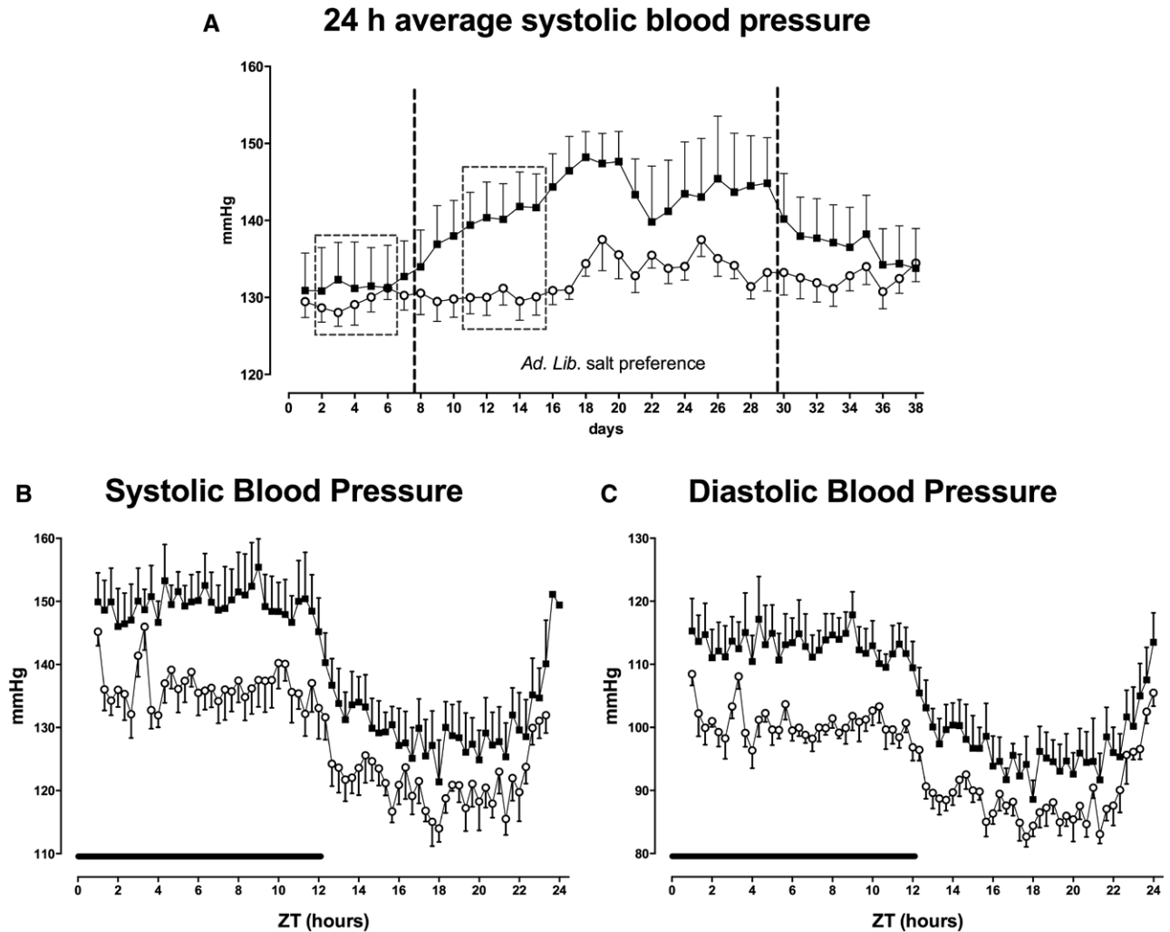
Figure 1. Salt sensitivity in Hsd11b2 .BKO mice. Blood pressure was measured in conscious, unrestrained Hsd11b2 .BKO ( n=6 ; filled squares) and control mice ( n=6 ; open circles) using radiotelemetry. All mice had access to 2 drinking bottles for the entire experiment; from day 8 to 29, 1 bottle contained 1.5% NaCl; at other times, both bottles contained water. A , 24-hour average systolic blood pressure. Data are mean \pm SEM. Two-way ANOVA reported a significant effect of genotype ( P<0.0001 ), of treatment ( P=0.013 ), and of the interaction between the main effects ( P=0.0021 ). Mesor, amplitude, and acrophase were calculated by cosinor analysis (Figure I and Table II in the online-only Data Supplement) of nonaveraged data obtained over consecutive days indicated by the boxes. Systolic blood pressure ( B ) and diastolic blood pressure ( C ) measured every 20 minutes over a 24-hour period. The black line indicates subjective night (7 PM to 7 AM local time). Data are group mean \pm SEM, generated by averaging each mouse over 5 consecutive days of recording. Mesor, amplitude, and acrophase were calculated by cosinor analysis (Table II in the online-only Data Supplement). ANOVA indicates analysis of variance; and SEM, standard error of the mean.
