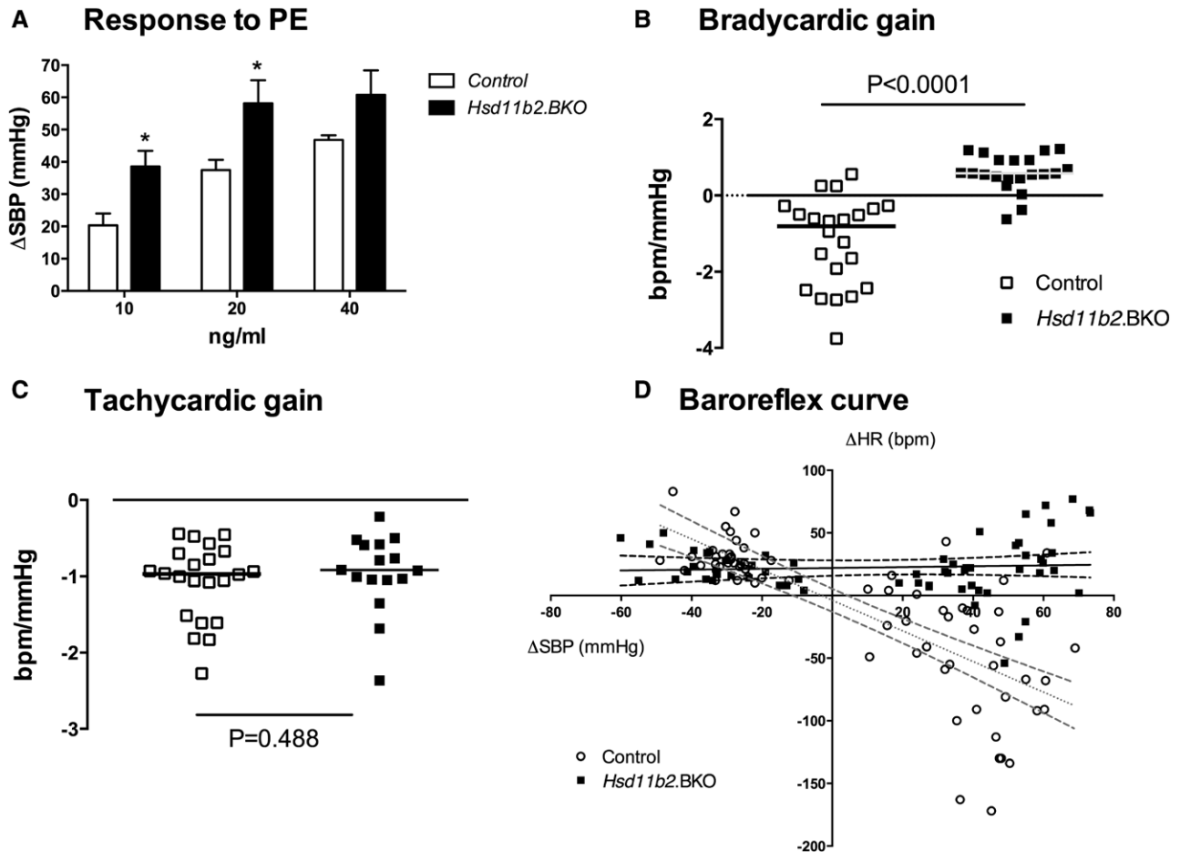
Figure 5. Baroreceptor reflex function. The baroreflex was measured pharmacologically in anesthetized Hsd11b2.BKO mice (filled squares; n=10 mice/63 responses) and controls (open circles; n=9 mice; 71 responses) mice. A , The mean change in systolic blood pressure ( \Delta SBP) in response to intravenous injection of phenylephrine. Two-way ANOVA reported a significant effect of dose ( P<0.0001 ) and genotype ( P=0.0002 ). Planned comparisons were made comparing each dose between genotypes. *P<0.05 . The baroreflex gain during intravenous injection of phenylephrine ( B ) and during intravenous injection of sodium nitroprusside ( C ); individual data points are shown and the median compared by Mann-Whitney test, with P values as indicated. D , The baroreflex curve showing individual data points for the change in heart rate ( \Delta HR) in response to induced changes in systolic blood pressure ( \Delta SBP). There was a significant difference ( P<0.0001 ) between genotypes by Linear regression analysis. ANOVA indicates analysis of variance; and PE, phenylephrine.
