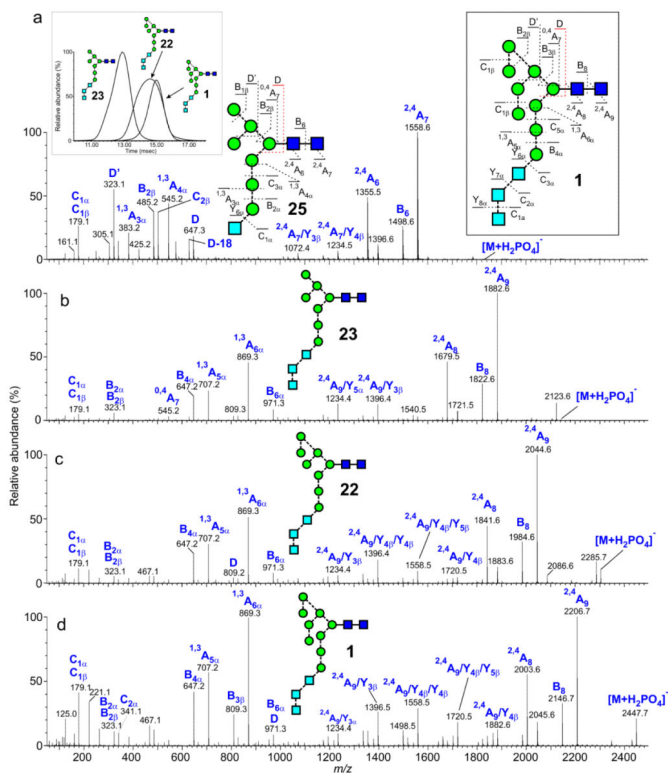
Figure 10. Negative ion CID spectra ( [M+HPO_4]^- ion) of: (a) Glc_1Man_7GlcNAc_2 ( 25 ). (b) Glc_3Man_7GlcNAc_2 ( 23 ). (c) Glc_3Man_8GlcNAc_2 ( 23 ) and (d) Glc_3Man_9GlcNAc_2 ( 1 ). Spectra b, c and d were from gp120 expressed in CHO cells in the presence of the \alpha -mannosidase inhibitor NB-DNJ. Inset 1 to panel a shows the ATD profiles for Glc_3Man_{7-9}GlcNAc_2 , Inset 2 shows the fragmentation of Glc_3Man_9GlcNAc_2 ( 1 ).
