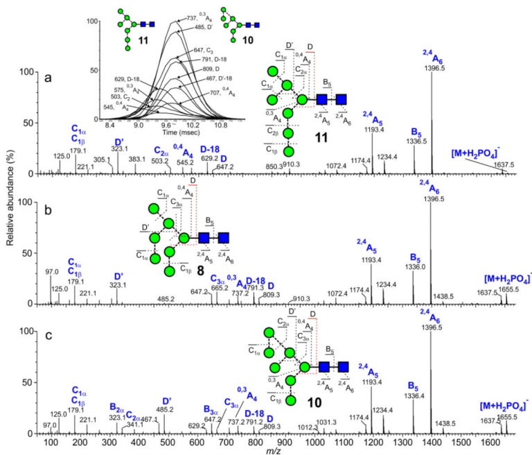
Figure 6. (a) Negative ion CID spectrum ( [M+H_2PO_4]^- ion) of Man_7GlcNAc_2 (d1d1 isomer, 11 , from porcine thyroglobulin). (b) Negative ion CID spectrum ( [M+H_2PO_4]^- 8 , from gp120, (JRCSF)). Negative ion CID spectrum ( [M+H_2PO_4]^- ion) of Man_7GlcNAc_2 (d1d2 isomer, 9 , from gp120, (JRCSF)). Negative ion CID spectrum ( [M+H_2PO_4]^- ion) of Man_7GlcNAc_2 (d1d3 isomer, 10 , from gp120). The inset to the first panel shows single ion plots of the 6-antenna-specific ions (smoothing algorithm, mean 2 \times 2 ) showing the presence of the minor isomer 11 . The spectrum in panel c was, thus, from the right-hand portion of the ATD peak.
