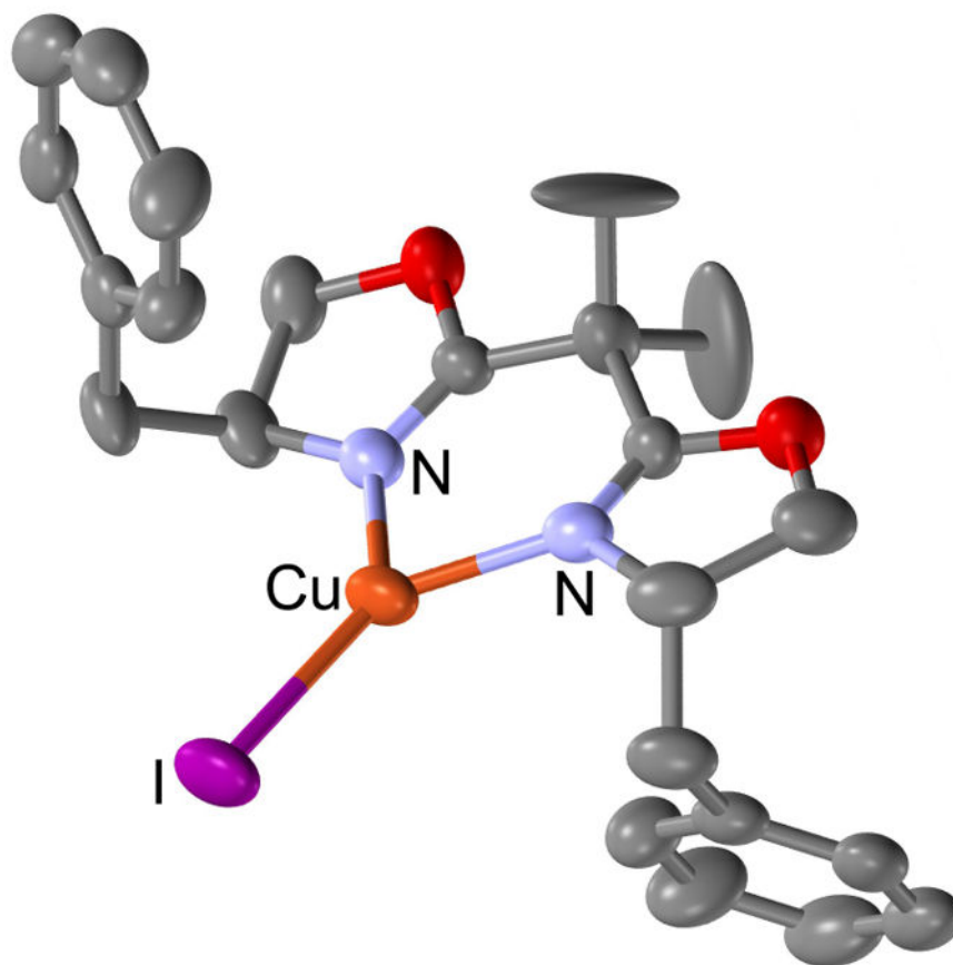
Figure 2. Molecular diagram of [( S,S )-BnBox]CuI with ellipsoids at 30% probability. H-atoms omitted for clarity.
