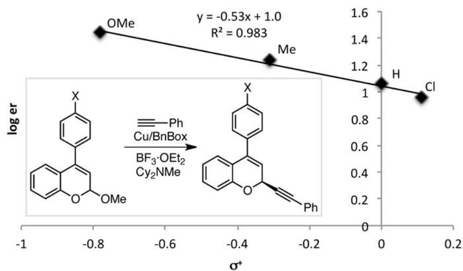
Figure 1. Hammett Plot of Substituent Effects of 4-Aryl-Substituted Chromene Acetals vs. Enantioselectivity
