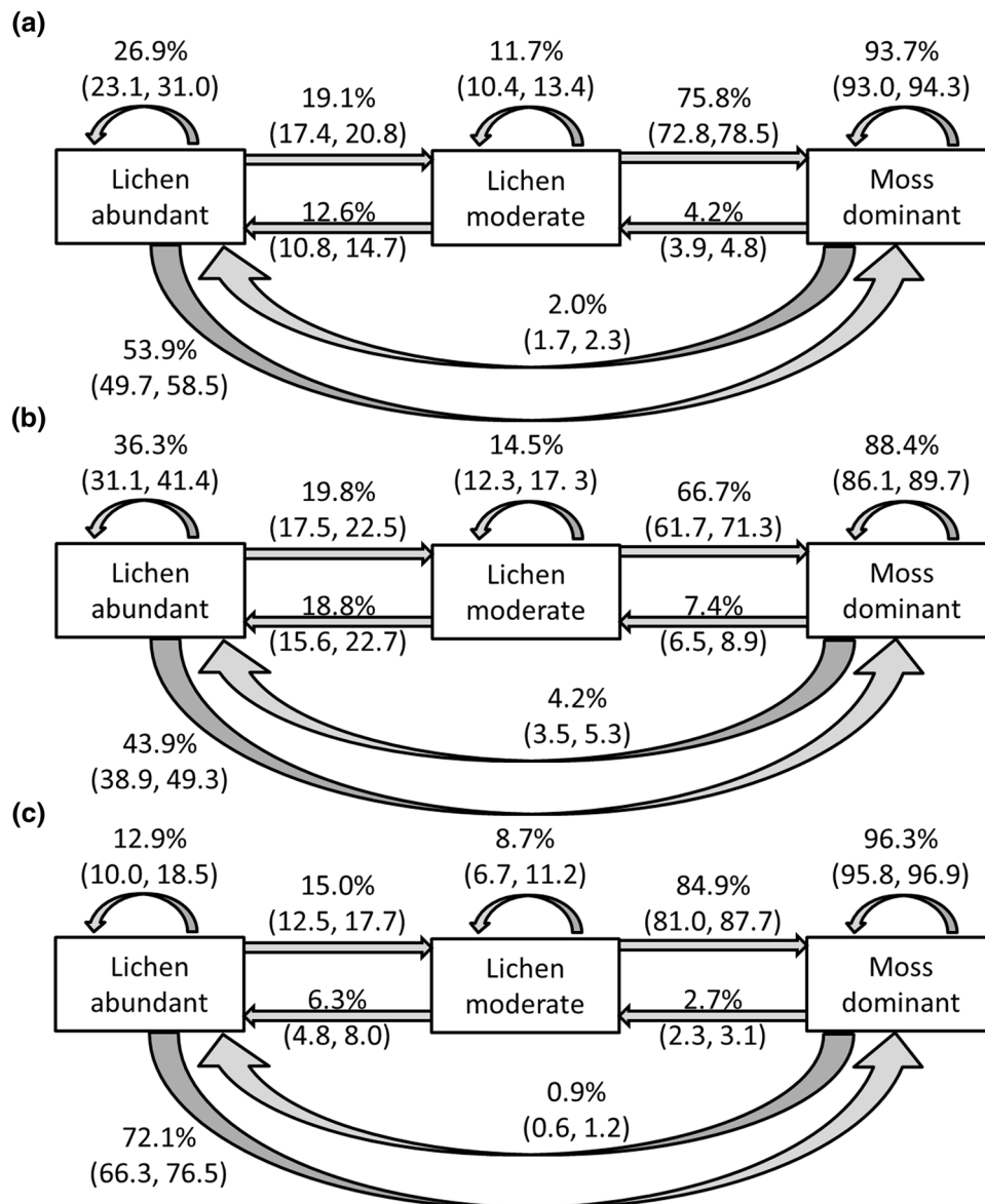
Fig. 4 The probability and confidence interval (in brackets ) that a sample plot has changed from one forest class to another class after 30 year for a all forest plots, b plots in open forest (basal area <15 \text{ m}^2 \text{ ha}^{-1} ) and c plots in dense forest (basal area \geq 15 \text{ m}^2 \text{ ha}^{-1} ), respectively. Lichen abundant ( >50 \% cover of ground lichen), Lichen moderate ( 25\text{--}50 \% cover of ground lichens) and moss dominant ( \leq 25 \% cover of ground lichens). The probabilities and confidence intervals are the results of a multi-state model
