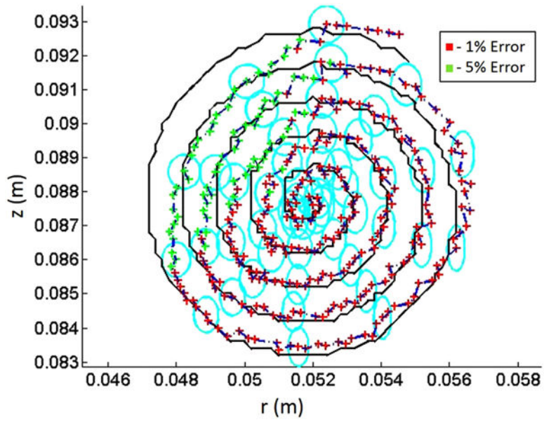
Fig. 6. Simulated motion of a capsule along a spiral trajectory in the center of \mathcal{G}^I . The black line represents the reference trajectory, while the crossed line shows the capsule position estimated by applying the Jacobian-based iterative method. The cyan ellipses represent the ellipsoid of localization uncertainty due to MFS noise. Colors in the crossed line express the relative error in position detection for the radial component.
