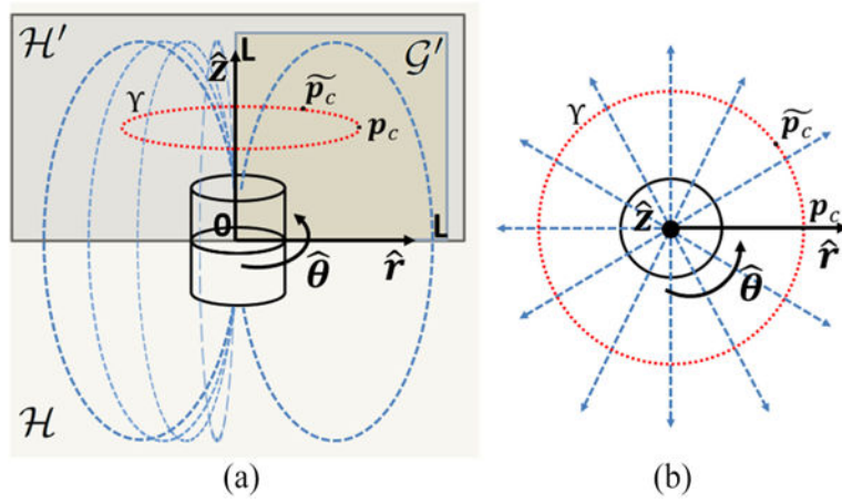
Fig. 3. Schematic view of the magnetic field distribution for a cylindrical axially magnetized permanent magnet. (a) View of the \mathcal{H} planes, its subset \mathcal{H}' , and the domain \mathcal{G}' . (b) Radial distribution of the magnetic field on the plane [\hat{r}, \hat{\theta}] .
