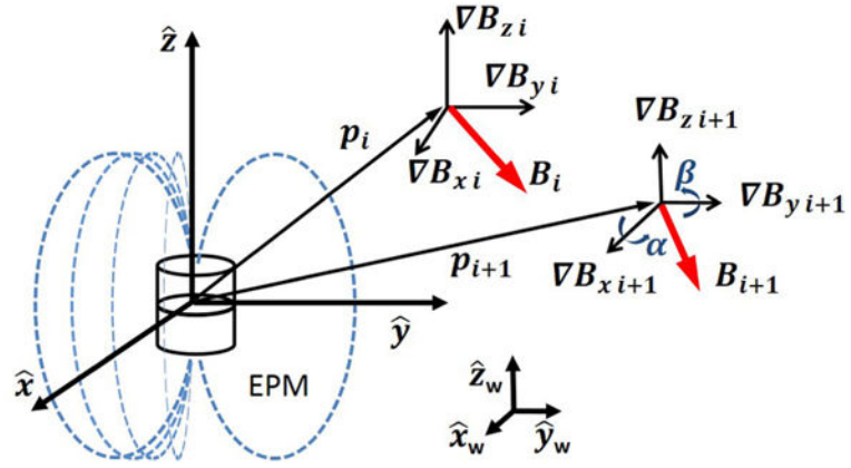
Fig. 1. Schematic representation of the source of magnetic field (EPM in the figure) and two sequential positions (i.e., \mathbf{p}_i and \mathbf{p}_{i+1} ) of the capsule to be localized. The capsule orientational angles yaw and pitch are referred to as \alpha and \beta , respectively.
