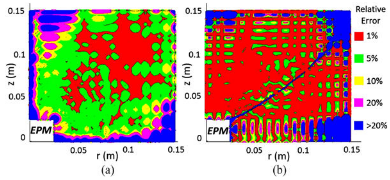
Fig. 4. Relative error for the (a) radial and (b) axial magnetic field estimated by the MDR within \mathcal{G}' .
