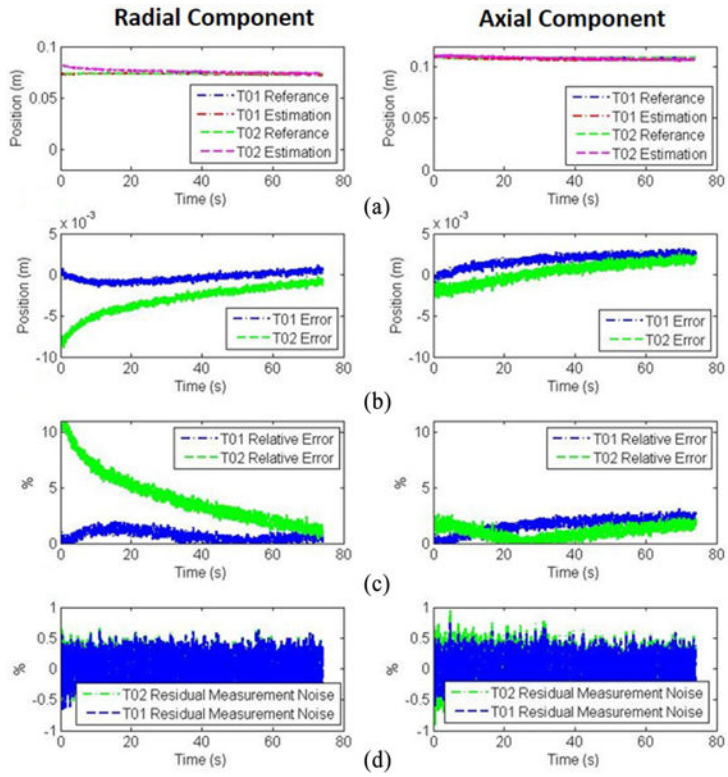
Fig. 9. Results for the steady-state positional drift experiment (T01) and for the initialization error evaluation (T02) with an initialization error of 10 mm. Both T01 and T02 results are evaluated for the radial (left column) and the axial (right column) component. (a) Reference position versus estimation. (b) Absolute positional errors. (c) Relative positional errors. (d) Residual measurement noise. The azimuth error is presented in Fig. 12.
