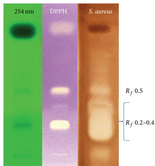
FIGURE 1: DPPH-radical scavenging and antibacterial (HP)TLC bioautographic assay. Active compounds corresponding to the different R_f are reported in Table 1.
