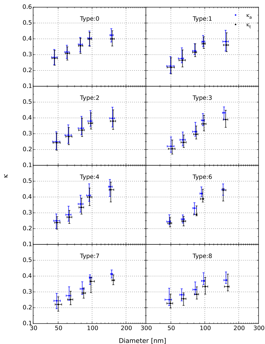
Figure 6. The averaged hygroscopic parameters ( \kappa_a , \kappa_t ) derived from CCN activation spectra under different weather-pollution types plotted against the critical diameter ( D_a or D_b , respectively). The data points are the median values corresponding to the weather-pollution type and given supersaturation, and the lower and upper bars represent the quartile error.
