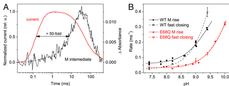
Fig. 3. (A) Laser flash-induced photocurrent generated by GtACR1 in a HEK293 cell (red line, left axis) and kinetics of the M intermediate in detergent-purified pigment monitored at 400 nm (thin black line) fitted with three exponentials (thick black dashed line). To correct for contribution of the formation and disappearance of the longer-wavelength (L-like) intermediate, the absorption changes at 410 nm were subtracted from those at 390 nm. (B) The pH dependencies of the rate of the M intermediate formation was monitored at 400 nm in purified pigments (solid lines, filled circles) and the rate of fast channel closing was measured by patch clamp in HEK293 cells (dashed lines, empty squares) in the WT (black symbols and lines) and the E68Q mutant (red symbols and lines). The data for M formation were pooled from five and two independent experiments in the WT and the mutant, respectively. The data for channel closing were obtained from ref. 3.
