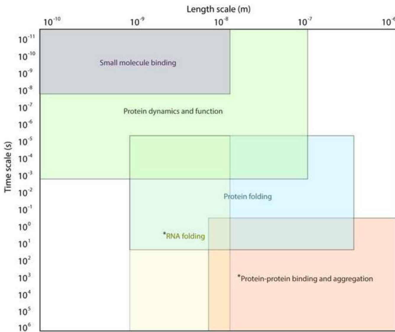
Figure 1. Length and time scales of molecular phenomena studied with DMD
