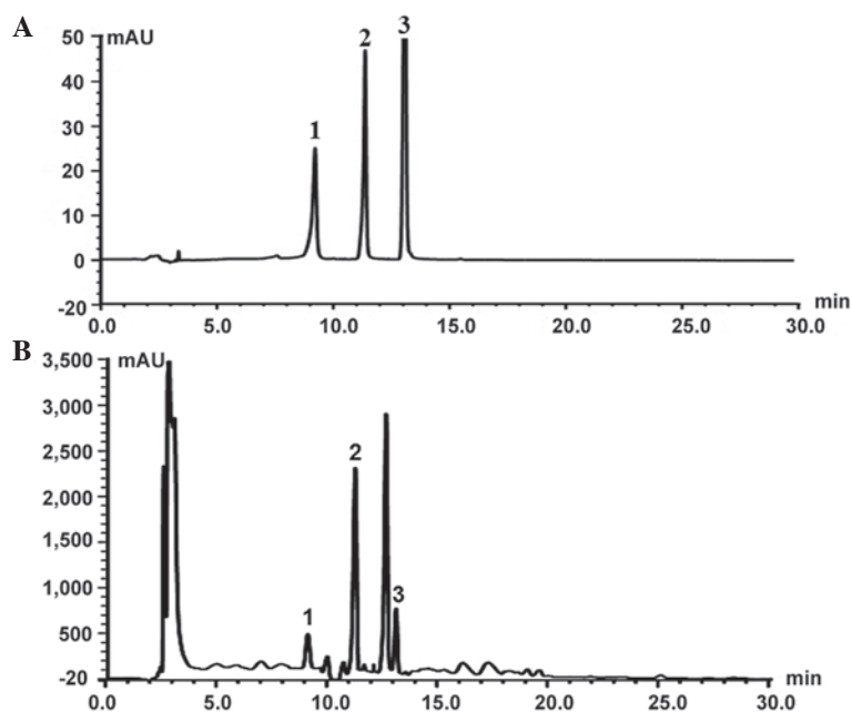
Figure 1. High-performance liquid chromatography profiles of (A) control solution and (B) Bauhinia championii (Benth.) Benth. extraction. Peak 1, myricetin; peak 2, quercetin; peak 3, kaempferol.
