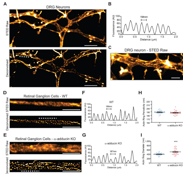
Figure 3. Lack of adducin gives rise of axon actin rings of increased diameter in RGCs (A) STED super resolution microscopy of DIV2 rat DRG neurons stained with SiR-actin; upper- raw images, lower- deconvolved images. Scale bar: 2 \mu m. The analysis of actin ring periodicity was performed in 16 independent axons in axonal segments of approximately 5 \mu m. (B) Representative fluorescence intensity profile graph of a 2 \mu m axonal segment of a DIV2 rat DRG neuron (obtained in the region highlighted by the dashed white line in Figure 3A, lower panel). (C) DIV2 DRG neurons present longitudinal actin filaments, highlighted with white arrowheads. Scale bar: 1 \mu m. (D and E) STED super resolution microscopy of WT (D) and \alpha -adducin KO (E) DIV19 RGCs; upper-raw images, lower- deconvolved images. Scale bars: 2 \mu m. (F-H) Analysis of the periodicity of axon actin rings in DIV19 RGCs from WT (F, H) and \alpha -adducin KO (G, H) neurons. Measurements were performed in deconvolved images. The analysis of the periodicity of axon actin rings was performed in WT n=28; \alpha -adducin KO n=33 independent axons in axonal segments of approximately 7 \mu m. (F and G) Representative fluorescence intensity profile graphs of 2 \mu m axonal segments highlighted by the dashed white lines in Figures 3D and 3E, respectively, lower panels). (I) Analysis of actin ring diameter in DIV19 RGCs from WT and \alpha -adducin KO neurons. p-value ***<0.001. WT n=28; \alpha -adducin KO n=32 axons. Graphs show mean \pm s.e.m.; each dot is the average measurement for a given individual axon.
