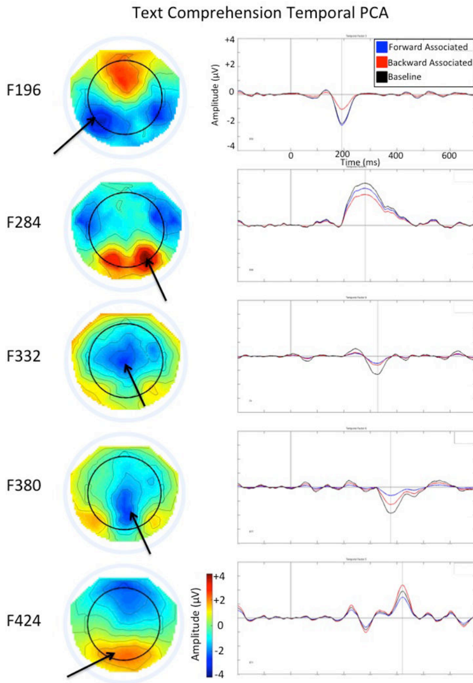
Figure 3. Temporal PCA components extracted from the text comprehension data. Principal components are illustrated in temporal order from top to bottom. The far left column indicates the time of peak activity of each factor (e.g., F196 = 196 ms). The next column illustrates topographic voltage maps, averaged across all conditions. The black arrow indicates the site of peak activity for each topographic map. The far right column contains the grand average factor waveforms for each condition, scaled to millivolts, with positive
