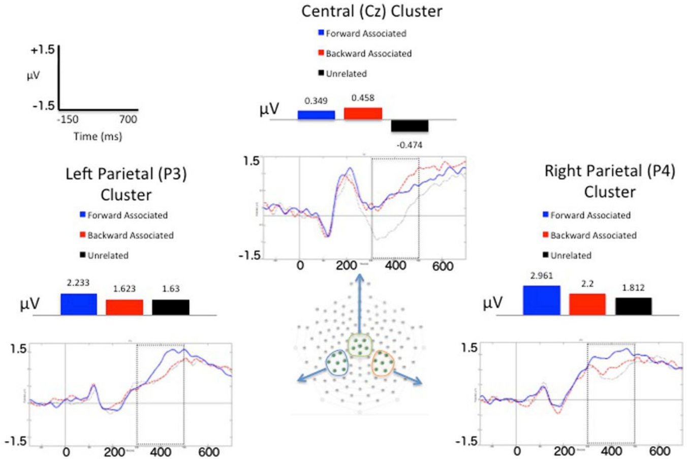
Figure 4. Waveforms and amplitude charts for the meaning judgment task ERP data. On the bottom is a schematic of the electrode net used in this study (anterior at the top), along with the three electrode clusters of interest (highlighted). On the right side of the schematic is the averaged waveform for the right (P4) parietal cluster, on the left side of the schematic is the averaged waveform for the left (P3) parietal cluster, and above the schematic is the averaged waveform for the central (Cz) cluster. The onset of the critical word is marked by the thin vertical line close to the left end of each waveform, and the 300–500ms time window of interest is indicated by the thicker black box further to the right end of the waveforms. The averaged amplitude data (in µV) across the 300–500ms time-window for each condition, and for each cluster, is shown above each respective waveform.
