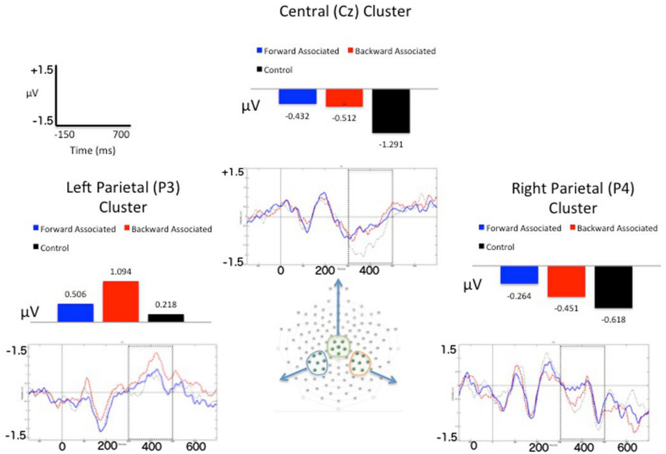
Figure 1. Waveforms and amplitude charts for the text comprehension task ERP data. On the bottom is a schematic of the electrode net used in this study (anterior at the top), along with the three electrode clusters of interest (highlighted). On the right side of the schematic is the averaged waveform for the right (P4) parietal cluster, on the left side of the schematic is the averaged waveform for the left (P3) parietal cluster, and above the schematic is the averaged waveform for the central (Cz) cluster. The onset of the critical word is marked by the thin vertical line close to the left end of each waveform, and the 300–500ms time window of interest is indicated by the thicker black box further to the right end of the waveforms. The averaged amplitude data (in \mu\text{V} ) across the 300–500ms time-window for each condition, and for each cluster, is shown above each respective waveform.
