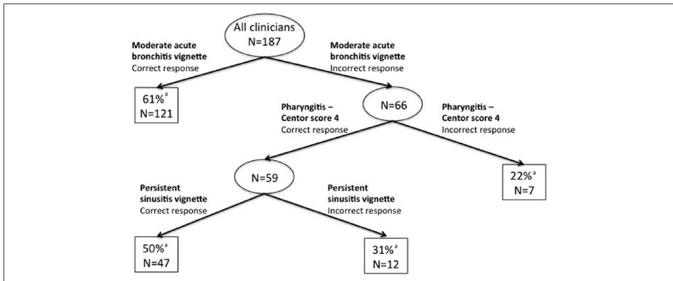
Figure 1. CART analysis of vignette-based ARI management to predict EHR-based performance on comprehensive management.
