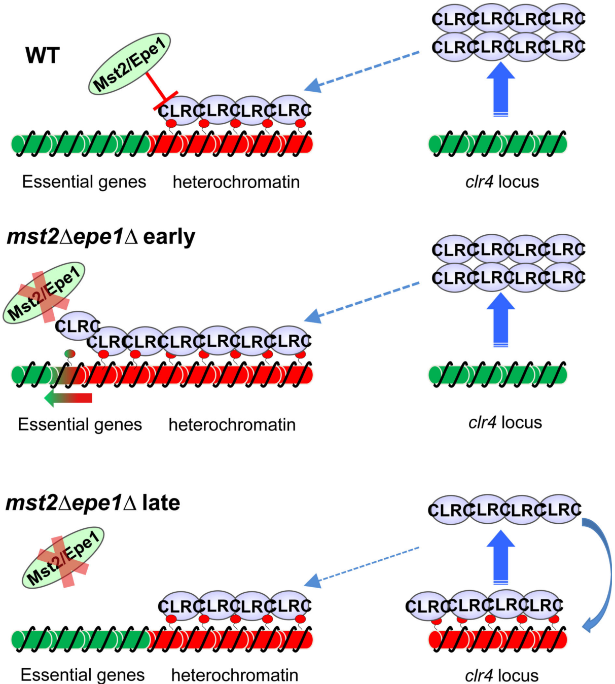
Figure 5. Heterochromatin-mediated epigenetic adaptation in fission yeast. The negative regulators of heterochromatin, Mst2 and Epe1, prevent promiscuous heterochromatin spreading in wild type cells. However, in mst2 epe1 cells, uncontrolled heterochromatin spreading inactivates essential genes, resulting in severe growth defects during early stage of development. Gradually, cells form heterochromatin at the clr4 + locus to reduce Clr4 expression levels, resulting in a new equilibrium that maintains heterochromatin at critical
