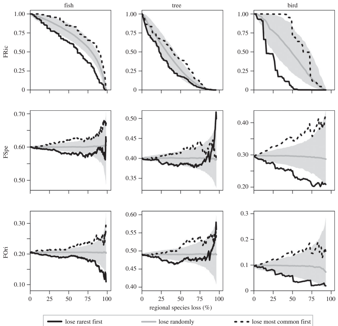
Figure 2. Impact of regional species extinction on the functional structure (functional richness, FRic; specialization, FSpe; and originality, FOr) of three tropical assemblages: stream fish from the Brazilian Amazon, rainforest trees from French Guiana, and birds from the Australian Wet Tropics. Rarest species sequential loss (black solid line) is compared with the opposite scenario where most common species are lost first (black dashed line) and with a null scenario simulating a random sequential extinction (grey line indicates the median of this scenario among 1 000 replicates and the 95% confidence interval is represented as the shaded area). Due to computation constraints the maximum species removals from the regional pools of fish, trees, and birds were, respectively, 99%, 96%, and 93%.
