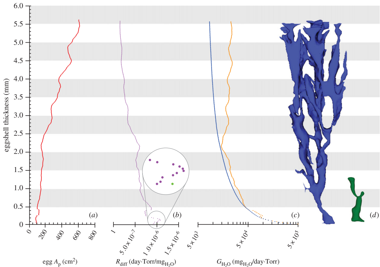
Figure 3. Egg pore area ( A_p ), diffusive resistance ( R_{\text{diff}} ) and water vapour conductance ( G_{\text{H}_2\text{O}} ) variation through the shell thinning of a 5.6 mm eggshell from Sanagasta. (a) A_p of each shell segment. (b) R_{\text{diff}} of each shell segment (dark grey; purple in the online version; based on Fick's law) and the inner aperture (light grey; green in the online version; based on Stefan's law). (c) G_{\text{H}_2\text{O}} at each thickness estimated through equation (4.1) (light grey; orange in the online version) and derived from R_{\text{diff}} (dark grey; blue in the online version); see Material and methods. Data are listed in the electronic supplementary material, S2. (d) Scaled Sanagasta pore set (left) and Auca Mahuevo layer 4 pore canal (right). Restoration of the Auca Mahuevo pore canal based on Grellet-Tinner et al. [5]. (Online version in colour.)
