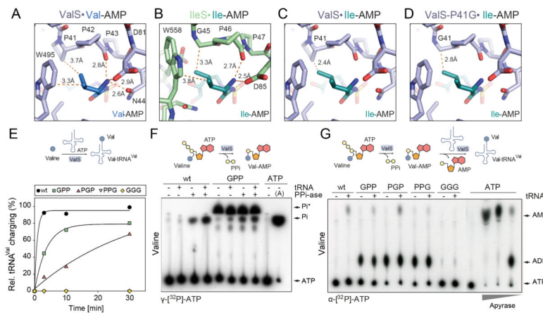
Fig. 2. PPP at the active site of ValS is required for efficient tRNA charging
