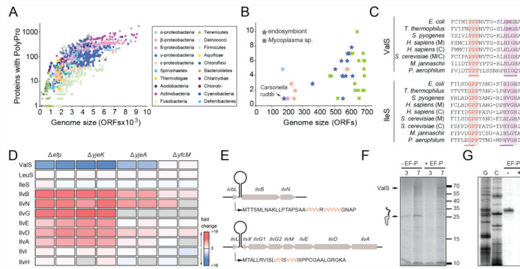
Fig. 1. A conserved proline triplet in ValS confers EF-P dependence for expression (A) Scatter-plot illustrating the total number of polyproline-containing proteins relative to genome size [in terms of open reading frame (ORF) number] of species within different bacterial phyla. (B) Zoom of (A) highlighting bacteria with the smallest genomes. (C) Sequence alignment illustrating the conservation of PPP and GPP in Val- and Ile-tRNA synthetases, respectively, across the three domains of life, compared with the highly conserved “HIGH” motif. (D) Heat map representation of changes in expression levels in vivo (blue, down-regulated; red, up-regulated; white, unchanged; grey, not identified or quantified) of selected proteins when comparing efp , yjeA , yjeK and yfcM strains against a wildtype E. coli internal standard. Data from two biological replicates taken from (Peil et al., 2013). (E) Schematic illustration of the gene arrangement of the ilvL-BN and ilvL-GMEDA operons, with the corresponding sequence of the leader peptides IbvL and IlvL. Valine residues essential for attenuation are shown in red. (F) Autoradiograph of SDS-PAGE monitoring the in vitro translation at 3 min and 7 min of ValS, in the absence (-EF-P) and presence of EF-P (+EF-P), with full-length (FL) ValS and peptidyl-tRNA (25 kDa) as indicated. (G) Toe-printing of ValS in the absence (-) and presence (+) of active EF-P. G and C sequence lanes are included.
