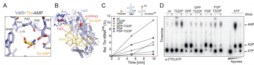
Fig. 3. PPP at the active site of ValS is required to prevent Thr-tRNA Val formation.
