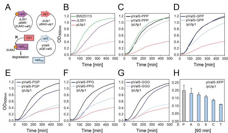
Fig. 4. The proline triplet of ValS is required for viability of E. coli .
