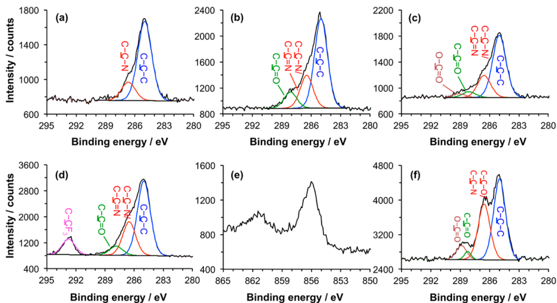
Figure 2. XPS data for APTES films following surface chemical reactions. (a) C 1s spectrum of an as-prepared film. (b) C 1s spectrum after incubation with glutaraldehyde solution. (c) C 1s spectrum after reaction of the aldehyde-functionalized surface with ABNTA. (d) C 1s spectrum after reaction of the aldehyde-functionalized surface with trifluoroethylamine. (e) Ni 2p spectrum after incubation of the NTA-functionalized surface with nickel chloride solution. (f) C 1s reference spectrum obtained for SAM of an NTA-terminated oligo(ethylene glycol) derivatized alkythiolate on gold.
