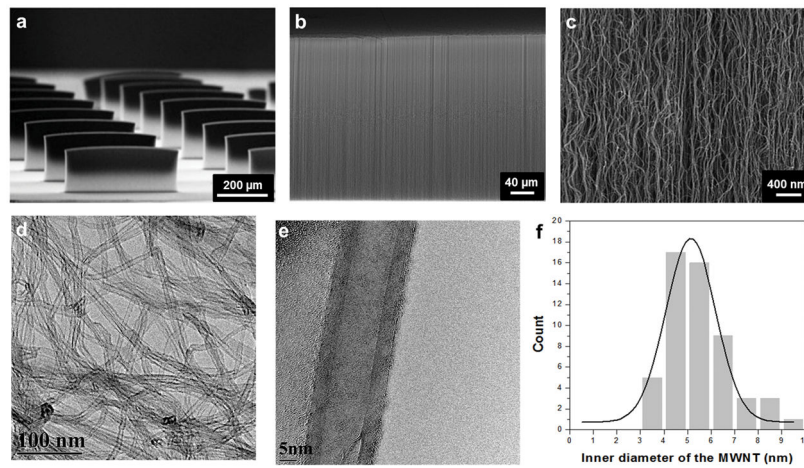
Figure 2. SEM images of (a) vertically aligned CNT forests (width: 460 \mu\text{m} and height: 300 \mu\text{m} ), (b–c) magnified parts of the CNT forest surface. (d & e) HRTEM images of multiple and individual MWNTs isolated from the CNT forest. (f) Diameter distribution of the MWNTs in the CNT forests.
