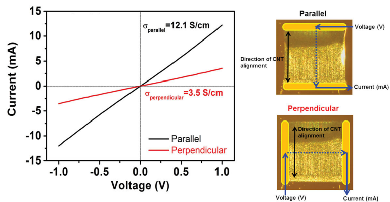
Figure 3. Two-point probe I-V curves from the CNT microelectrodes in parallel and perpendicular configurations relative to the nanotube alignment direction of CNT microelectrodes were measured. Au contacts were deposited at the edges of the CNT microelectrodes.
