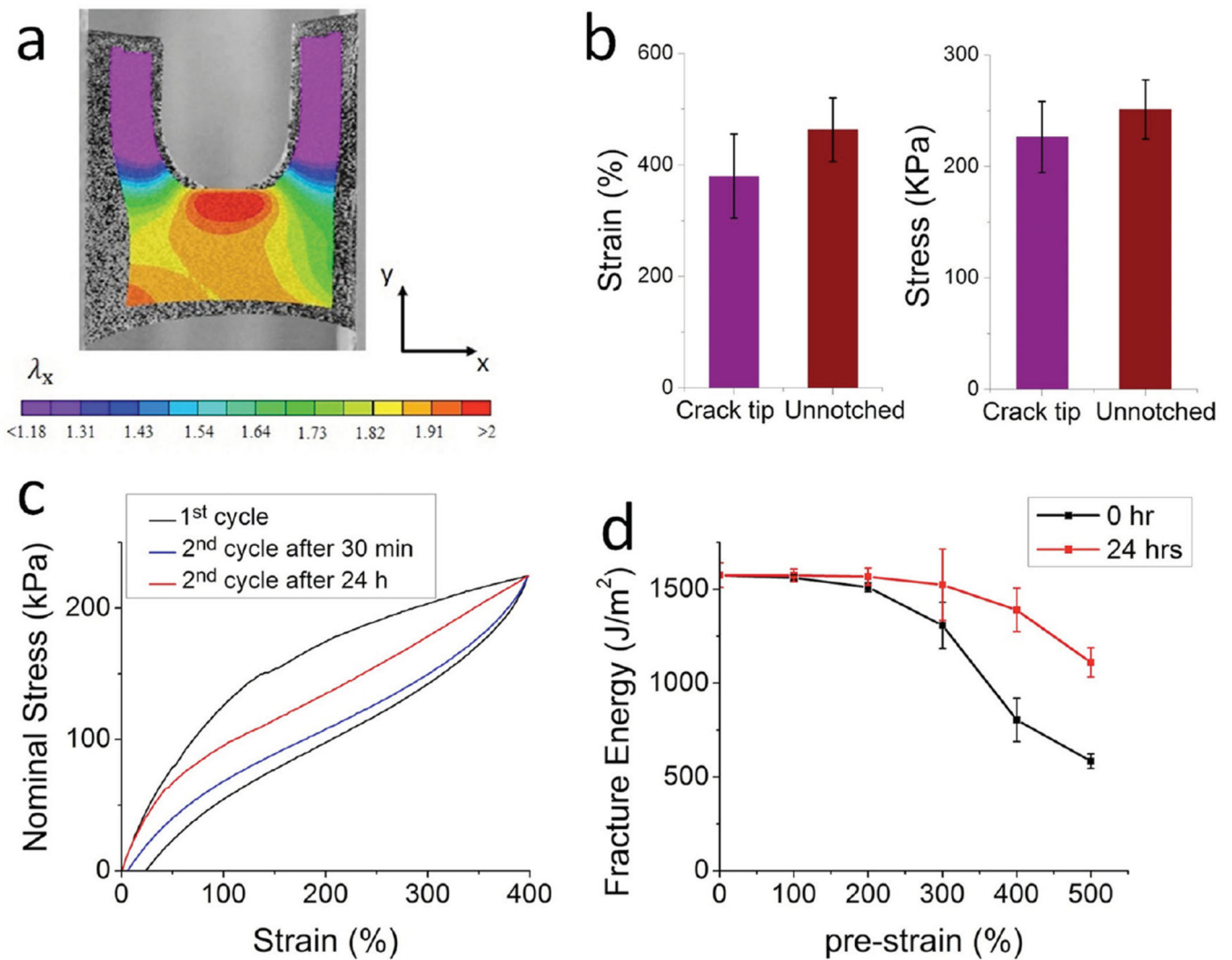
Figure 2. Mechanical properties of the hydrogel. a) Stretch along x -direction in a notched sample of the hydrogel under pure-shear test. b) Comparison of the critical strain and stress at the crack tip before crack propagation and the failure strain and stress of a sample without notch under pure-shear tension. c) Stress–strain hysteresis of the hydrogel under the first and second cycles of deformation. The sample was stored in a humid chamber at 37 °C for 5 min or 24 h between the two cycles of deformation. d) Fracture energies of hydrogels predeformed to different strains. The fracture energies were measured right after the predeformation or after storing the hydrogel in a humid chamber at 37 °C for 24 h.
