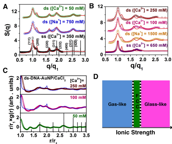
Figure 2. Structure of DNA coated AuNP assemblies. (A, B) SAXS-derived S(q) for DNA-grafted-AuNP aggregates (circles) along with simulations based on FCC lattices (red lines). For reference, the expected peak positions and relative intensities for Bragg reflections from ideal FCC lattices are shown (A, vertical black lines). The labels ss and ds correspond to ss-DNA-AuNP and ds-DNA-AuNP, respectively. (C) Representative radial distribution functions for ds-DNA-AuNPs in \text{CaCl}_2 as a function of \mu_s along with the expected positions and relative populations ( P/12 ) for neighbors in a FCC lattice (black lines). For visual comparisons, g(r) is plotted against normalized radial distance r/r_1 . Here, r_1 = d_{\text{NN}} represents the nearest-neighbor interparticle distance. Monte Carlo simulations (section 1.4 in the Supporting Information) for g(r) based on random close packing (RCP) of hard spheres (blue lines) reasonably describe the experimental g(r) for \mu_s much higher than \mu_t . (D) Schematic of the observed changes in colloidal packing as a function of ionic strength.
