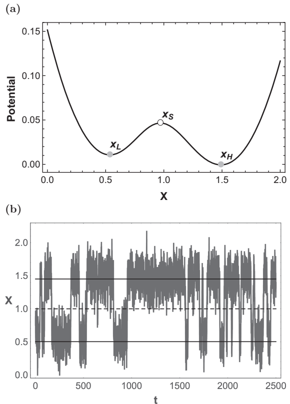
FIG. 1. Lake eutrophication model (example 1). (a) The potential function for Eq. (1). The horizontal axis is the scaled nutrient (phosphorous) concentration and the vertical axis is the (dimensionless) potential. Gray disks are stable equilibria, and the white disk is an unstable (saddle) equilibrium. The dynamics of the system can be represented as a ball rolling on the surface specified by the potential function. Note that the basin around x_H is deeper than that around x_L . (b) A realization of Eq. (3), which models nutrient concentration, x , as a function of time, t . Variables are scaled, so the units are dimensionless. Integration was performed with the Euler-Maruyama method and \Delta t = 0.005 . The solid lines corresponds to stable equilibria x_L (lower) and x_H (higher) for the deterministic skeleton. The dashed line corresponds to the saddle point x_S of the deterministic skeleton. Note that the realization spends more time near x_H than near x_L .
