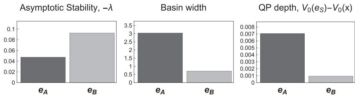
FIG. 5. (a) A schematic diagram of the relationship between various concepts of stability, as related to the quasi-potential and V_0 . (b) A comparison of three different metrics of stability for the system (8).
