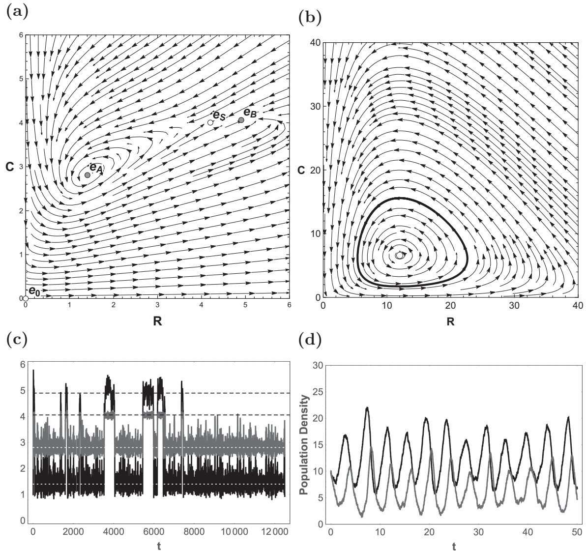
FIG. 2. (a) Stream plot for the deterministic skeleton of the consumer-resource model in example 2. Unstable equilibria are white disks and stable equilibria are gray disks. The unstable equilibrium e_p is not shown, but would appear on the x -axis to the right of where the graph is truncated. Variables are scaled, so the units are dimensionless. Lines and arrows show the direction of trajectories for Eq. (8) in the absence of noise. (b) Similar stream plot for the deterministic skeleton of the consumer-resource model in example 3. The white disk is an unstable equilibrium and the gray line is a stable limit cycle. (c) A realization of Eq. (8) for example 2. Integration was performed with the Euler-Maruyama method and \Delta t = 0.025 . Resource population density is black and consumer population density is gray. The dotted white lines correspond to the equilibrium e_A , and the dashed black lines to the equilibrium e_B . (d) A realization of Eq. (15) for example 3, with \sigma = 0.8 . Integration was performed with the Euler-Maruyama method and \Delta t = 5 \times 10^{-4} . Resource population density is black and consumer population density is gray.
