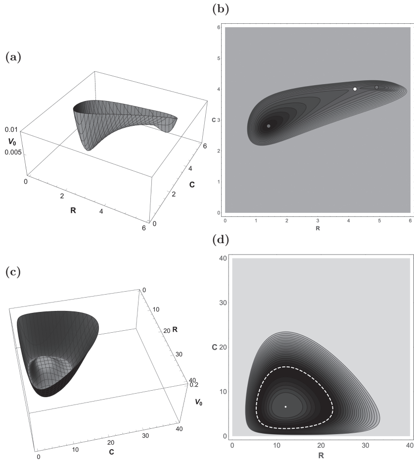
FIG. 3. (a) The quasi-potential function for the consumer-resource model, Eq. (8). Variables are scaled, so the units are dimensionless. Note that the quasi-potential surface is much deeper around \mathbf{e}_A than \mathbf{e}_B . The quasi-potential is truncated at 0.02 for display purposes; it continues to increase in the regions outside the plot. (b) Contour plot for the same model. The white disk is the saddle point \mathbf{e}_S . The gray disks are the stable equilibria \mathbf{e}_A and \mathbf{e}_B . (c) The quasi-potential function for Eq. (15). (d) Contour plot for the same model. The white disk is an unstable equilibrium, and the white dashed line is a stable limit cycle.
