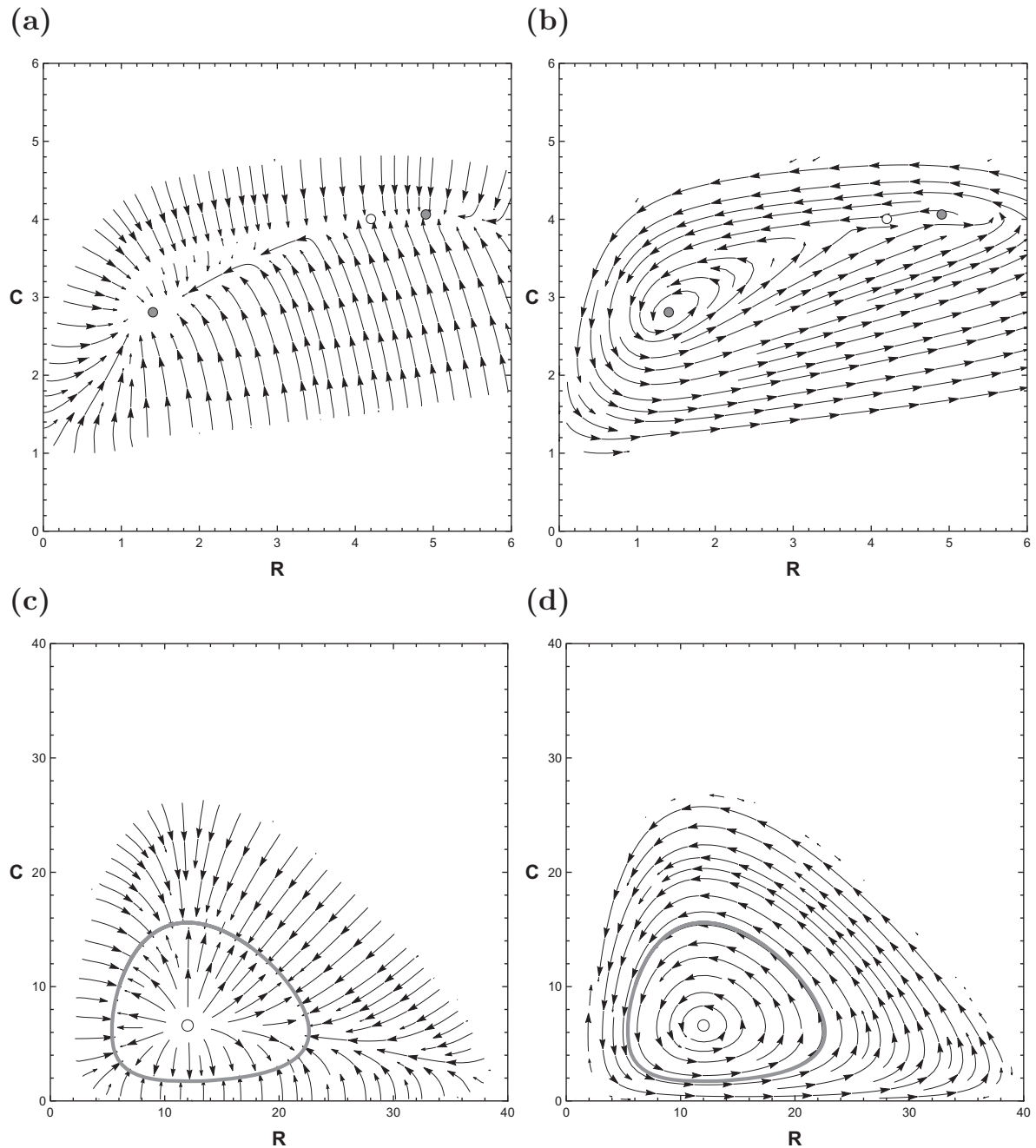
FIG. 4. (a) and (b) are the orthogonal decomposition of the deterministic skeleton of the system (8). (a) The “downhill” component, -\nabla V_0 . (b) The “circulatory” component, Q . Gray disks are stable equilibria. The white disk is an unstable equilibrium. (c) and (d) are the orthogonal decomposition of the deterministic skeleton of the system (8). The thick gray line is a stable limit cycle.
