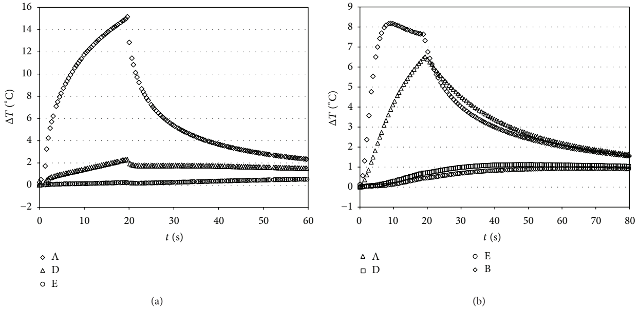
FIGURE 7: Characteristic temperature versus time curves caused by irradiation with Starlight PRO (Mectron) tested at a light intensity of 1000 (for 20 s) without (a) and with resin polymerization (b). A (1 mm from light source); B (bottom of the box); D (mesial); E (pulp chamber).
