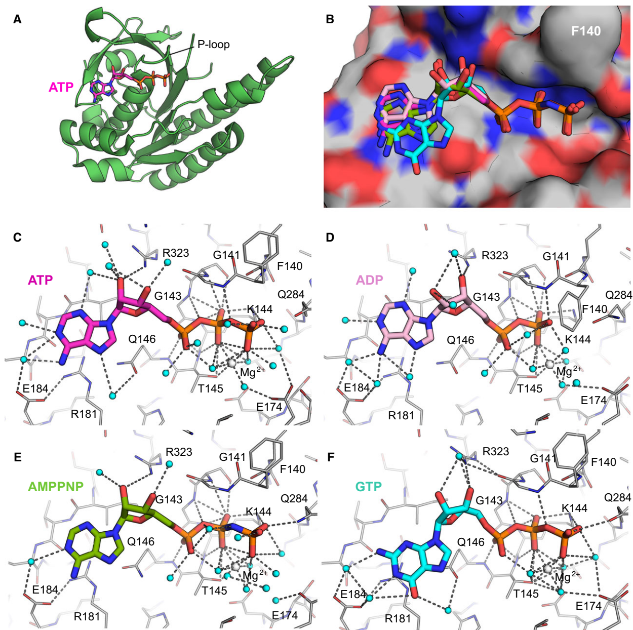
Fig. 4. Crystal structures of nucleotide-bound monomeric RadA. (A) Overview of RadA-ct bound to ATP. (B) Overlay of all nucleotides in superimposed RadA-ct complexes. Nucleotides are shown in stick representation: ATP (purple), ADP (pink), AMPPNP (green), GTP (cyan). Protein shown as surface molecule is that complexed with ATP, with F140 labelled to aid with orienting it with respect to the remaining figures. (C–F) Hydrogen bonding interactions between RadA-ct and ATP (C), ADP (D), AMPPNP (E) and GTP (F). Water molecules are shown as cyan spheres and Mg 2+ ions as white spheres. Colouring of nucleotides as in (B).
