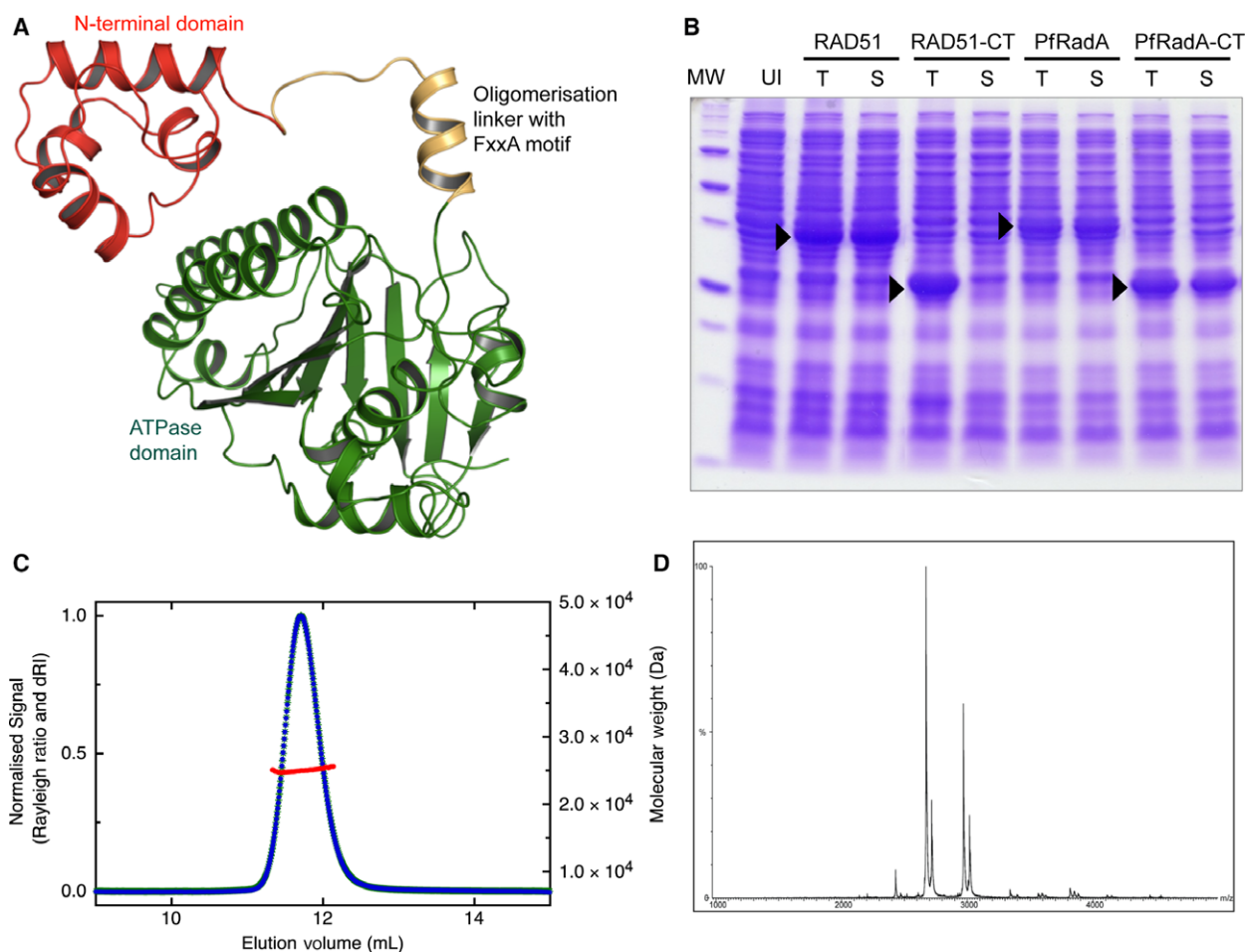
Fig. 1. C-terminal ATPase domain of Pyrococcus furiosus RadA is monomeric (A) Domain structure of a single protomer of full-length RadA from Pyrococcus furiosus (PDB: 1PZN) showing the different structural units in different colours (B) SDS/PAGE gel of E. coli expression tests for both full-length proteins and C-terminal domains of P. furiosus RadA and human RAD51; total lysate (T), soluble fraction (S) and uninduced control (UI). (C) Multi-angle laser light scattering chromatogram showing protein elution monitored by the change in refractive index (blue) and molecular weight calculated from light scattering data (red). (D) Nondissociative mass spectrum showing ions with mass/charge ratios consistent with a monomeric C-terminal RadA.
