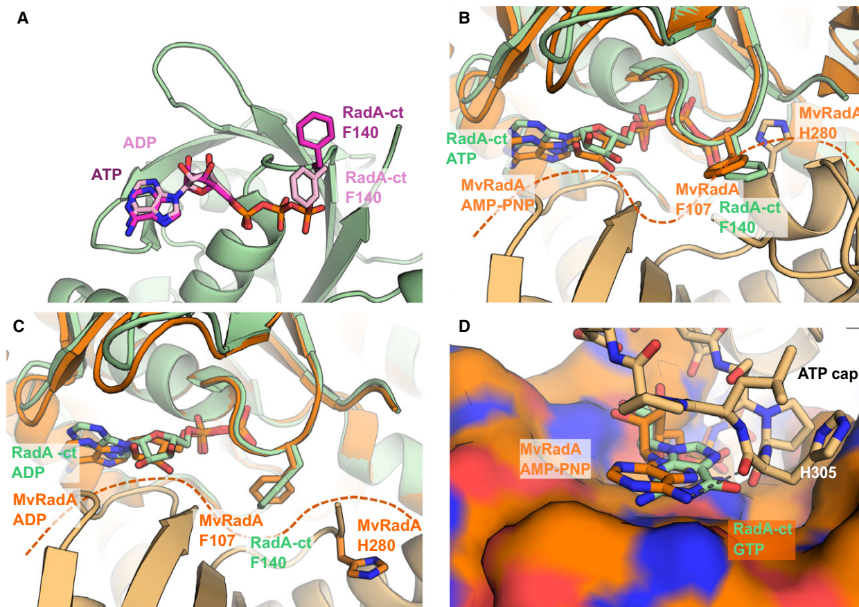
Fig. 5. Comparison of monomeric RadA-ct nucleotide complexes with filament structures of Methanococcus voltae RadA. (A) Superimposed nucleotide-bound RadA-ct structures with ATP and ADP. Nucleotides shown in stick representation – ATP (purple), ADP (pink). The F140 residue is shown in stick representation to illustrate the differing conformation between the ATP-bound (purple) and ADP-bound structures (pink). (B) Superimposed ATP-bound monomeric RadA-ct (light green) and AMPPNP bound to Methanococcus voltae RadA ( MvRadA ) oligomer with the adjacent RadA molecules coloured in darker and lighter orange (PDB: 2FPM). MvRadA residues and AMPPNP are shown in orange, PfRadA residues and ligand in light green. Superpositioning was done between RadA-ct and the MvRadA protomer shown on the top, and the interface between the two MvRadA molecules is indicated with a dashed line. (C) Superimposed ADP-bound RadA-ct and ADP-bound MvRadA molecules (PDB: 2FPK), coloured as in panel (B). (D) Superimposed structures of GTP-bound RadA-ct and AMPPNP-bound MvRadA oligomer (PDB: 2FPK). One of the protomers in the MvRadA oligomer is shown as molecular surface and the ATP loop of the adjacent protomer is shown as sticks. Hydrogen bond between main chain oxygen and the adenine N6-exoamino group of AMPPNP is shown as a dashed line.
