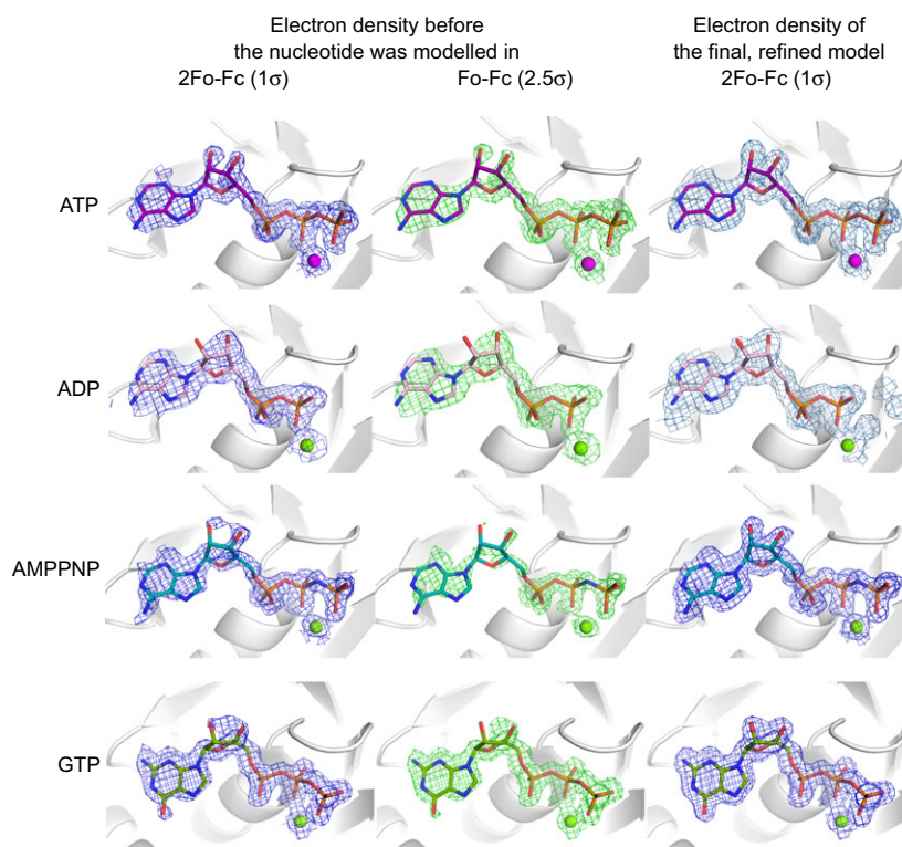
Fig. 3. Electron density maps of the bound nucleotides. Weighted 2FoFc and FoFc electron density maps shown in blue (countered at 1\sigma ) and green ( 2.5\sigma ), respectively in the left and middle columns for each of the nucleotides before the nucleotide was modelled into the structure. The right column shows the final weighted 2FoFc maps for each of the modelled nucleotides and their associated Mg^{2+} ions.
