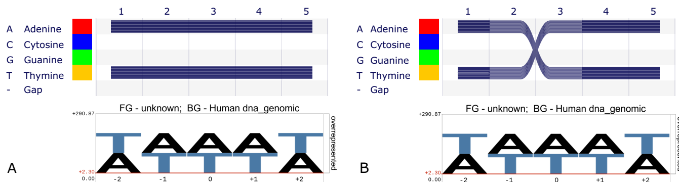
Figure 1. (A) Sequence Bundles (top) and pLogo (bottom) representation of an alignment of 1000 sequences with 500 instances of AAAAA and 500 instances of TTTTT . (B) The same visualizations rendered on a 1000 sequence alignment with 500 instances of AATT and 500 instances of TTAA . The pLogo representations in (A and B) are identical and reflect only the identical sitewise nucleotide frequencies in the two examples. (The different ordering of letters is a result of the chosen genomic background [human whole-genome].) Sequence Bundles clearly show the two sequence motifs in each case, because the nucleotides remain connected in the visualization.
