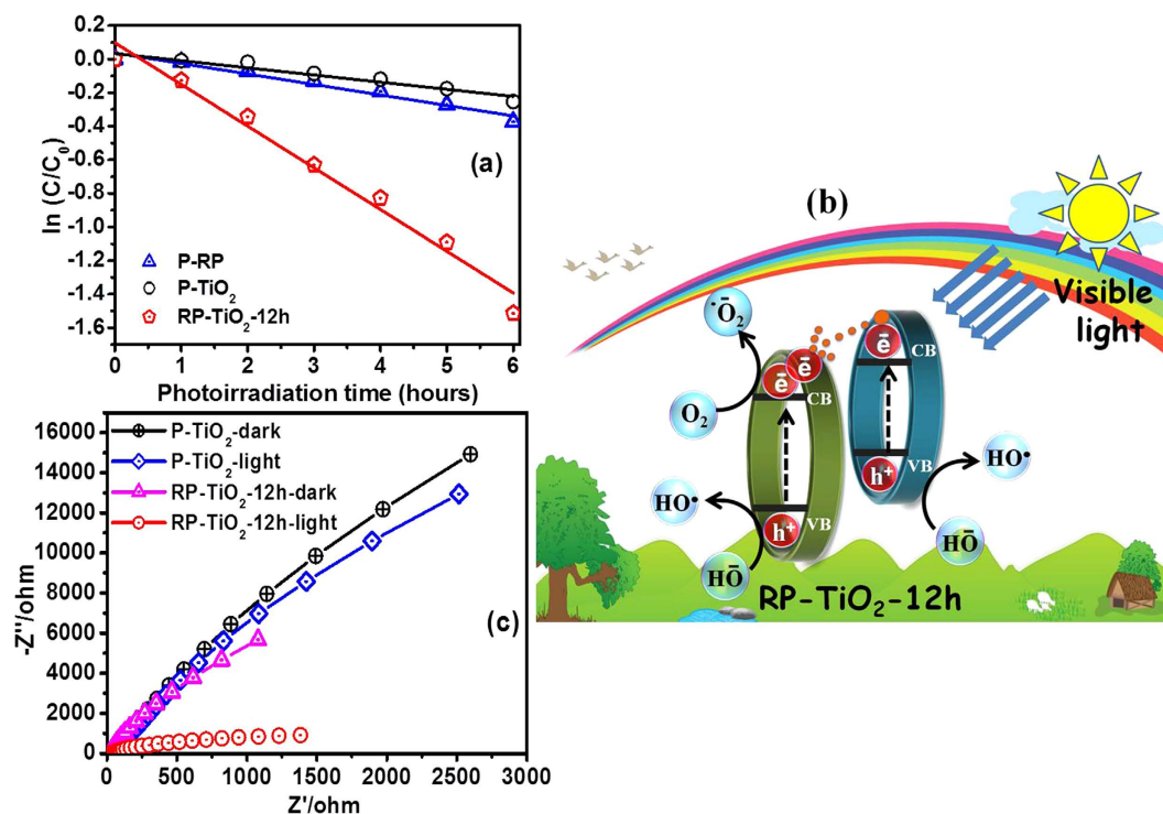
Figure 7. (a) Photodegradation kinetic plot of RhB as a function of the illumination time over P-TiO 2 and RP-TiO 2 -12 h nanohybrid photocatalyst, (b) proposed schematic diagram of the photoexcited electrons-holes generation, separation, and their transport process over the RP-TiO 2 -12 h photocatalyst interface under visible light illumination, and (c) Nyquist plots.
