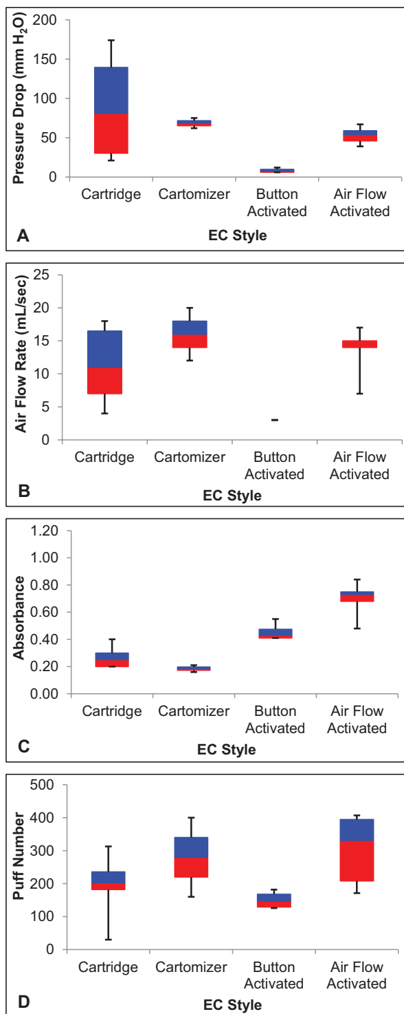
Figure 4. Comparison of performance properties across different generations of EC including EH (this figure can be seen in color online ). Four performance properties are summarized in box-whisker plots for cartridge models (Trtchounian et al., 2010), cartomizer models (Williams & Talbot, 2011), disposable button-activated models, and disposable airflow-activated models (current study). Each box shows the median, 75% percentile (blue box), 25% percentile (red box), and minimum and maximum values. The number of brands in each group was: six cartridge style, two cartomizer style, four button-activated disposable brands, and five airflow-activated disposable brands.
