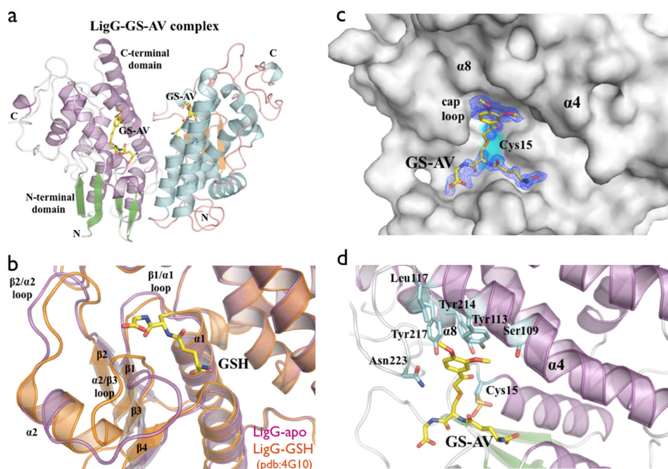
FIGURE 4. a , overall schematic representation of the LigG-GS-AV complex dimer. b , superposition of the GSH binding site of apo-LigG (magenta) and LigG-GSH (Protein Data Bank entry 4G10) (orange) structures (30). Significant conformational changes of the GSH binding site were observed on the loop regions at the N-terminal domain connecting the \beta 1/\alpha 1 , \beta 2/\alpha 2 , and \alpha 2/\beta 3 structural elements. c , molecular surface representation of the LigG monomer in complex with the GS-AV substrate analog. A feature-enhanced map (35) contoured at 1.0 \sigma is shown in blue around the GS-AV substrate analog (this molecule was omitted from the model to reduce bias). The position of the catalytic Cys 15 residue is highlighted in cyan. d , active site of the LigG-GS-AV complex. The glutathionyl moiety of the GS-AV substrate sits on the top of the four \beta -strands of the N-terminal thioredoxin domain. In addition, the AV moiety of the GS-AV molecule contacts the C-terminal \alpha -helical domain of LigG via residues Ser 109 , Tyr 113 , and Leu 117 on \alpha 4 , residues Tyr 214 and Tyr 217 on \alpha 8 , and Asn 223 on the cap loop region composed of the residues 220 GGGNG 224 .
