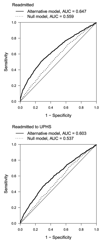
Fig. 1. ROC curves for 30-day all-cause readmission among Pennsylvania residents discharged from UPHS with a primary diagnosis of heart failure, 2005–2012, using the true (“readmitted”) and possibly misclassified (“readmitted to UPHS”) outcomes. The “null” model was based on sociodemographic characteristics and comorbid conditions diagnosed at discharge; the “alternative” model additionally included the number of admissions in the previous year.
