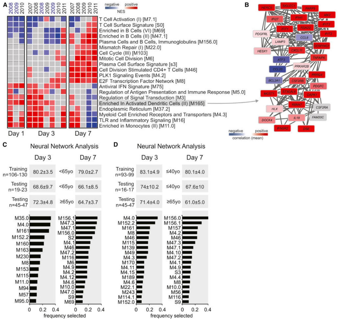
Figure 2. Signatures Associated with the Antibody Response Induced by TIV (A) Heat map of blood transcription modules (BTMs, rows) and TIV seasons (columns) whose activity at days 1, 3, or 7 after vaccination is associated with HAI response at day 28 after vaccination. Gene set enrichment analysis (GSEA, nominal p < 0.05 ; 1,000 permutations) was used to identify positive (red), negative (blue), or no (gray) enrichment of BTMs (gene sets) within pre-ranked gene lists, where genes were ranked according to their correlation between expression and HAI response. Seasons labeled in blue are from Franco et al. (2013) dataset. Modules shown are those consistently enriched in at least 70% of seasons on a given day. Abbreviation is as follows: NES, normalized enrichment score. (B) Genes in BTM M165; each “edge” (gray line) represents a coexpression relationship, as described in Li et al. (2014); colors represent the mean correlation for seven TIV seasons
