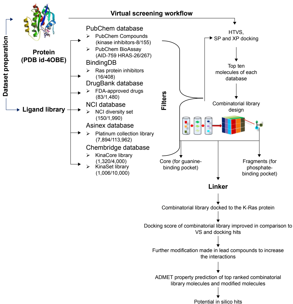
Figure 3 The workflow of implemented chemical database VS and combinatorial fragment-based approaches to design leads for the K-Ras protein.
