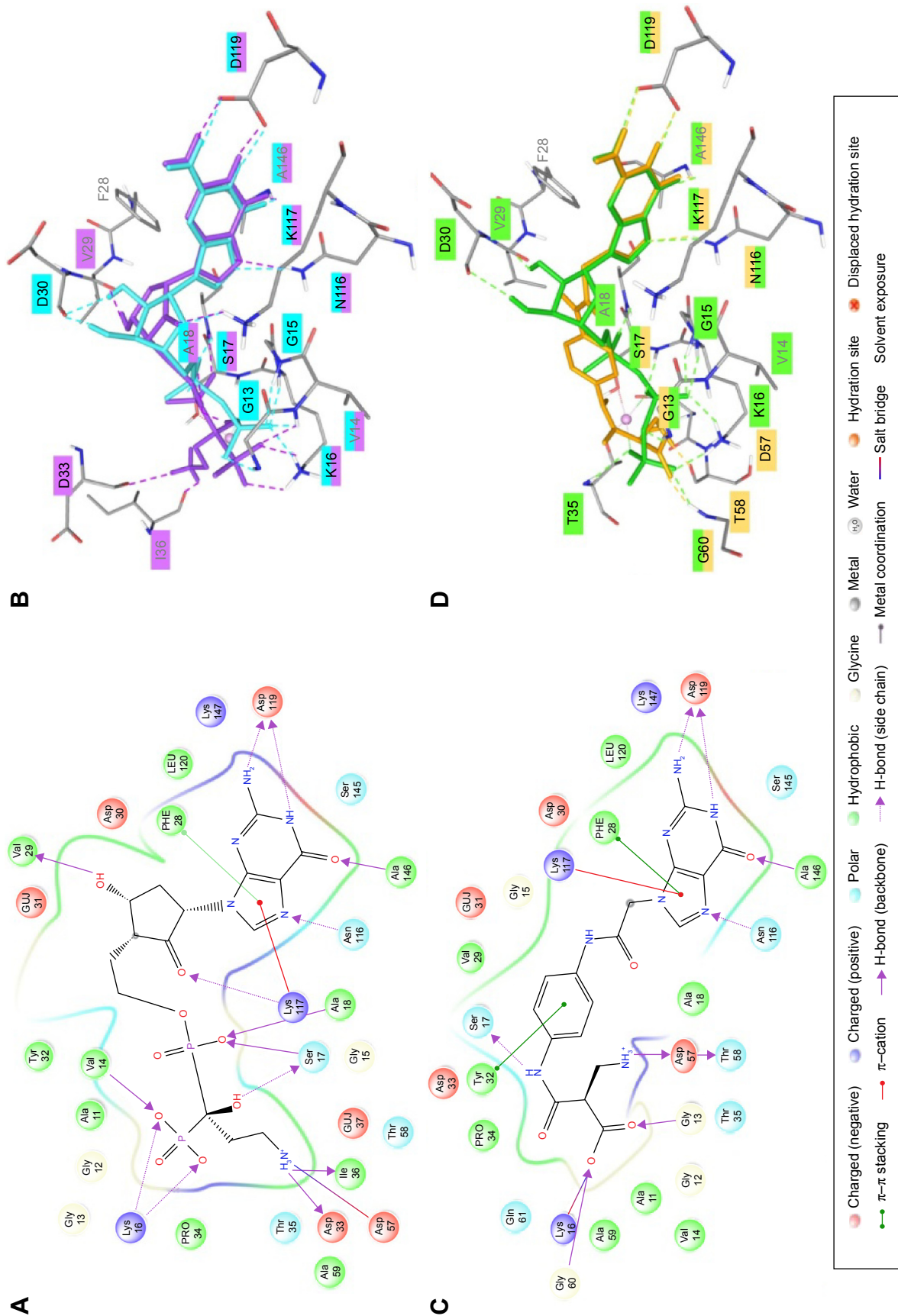
Figure 5 (A) Ligand interaction diagram of M3. (B) Superposition of GDP (cyan)-bound conformation and best-designed molecule M12 (amber)-bound conformation and best-designed molecule M12 (amber). (C) Superposition of M3 (purple). (D) Superposition of M3 (purple) and best-designed molecule M12 (green)-bound conformation and best-designed molecule M12 (amber). Abbreviations: GDP, guanosine diphosphate; GTP, guanosine triphosphate.
