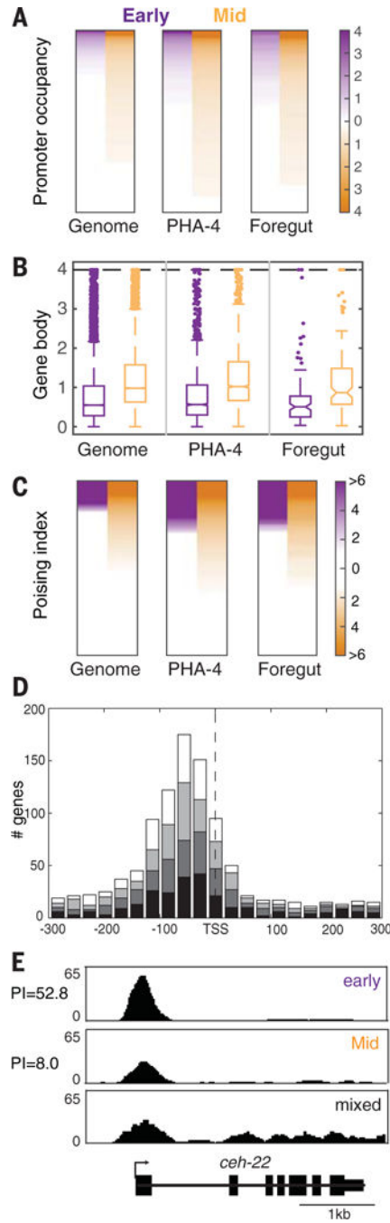
Fig. 2. Early embryos accumulate poised Pol II
