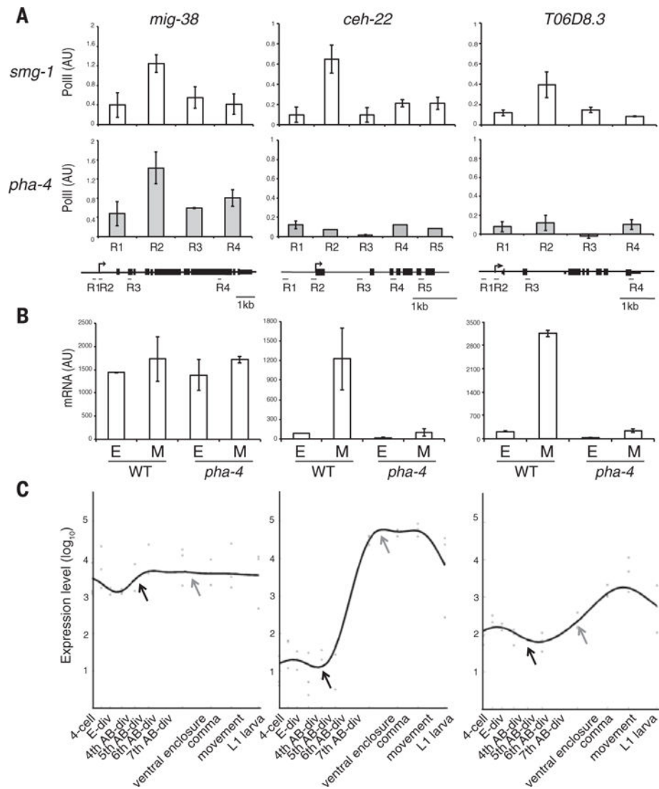
Fig. 3. PHA-4 is required for Pol II occupancy at foregut genes
