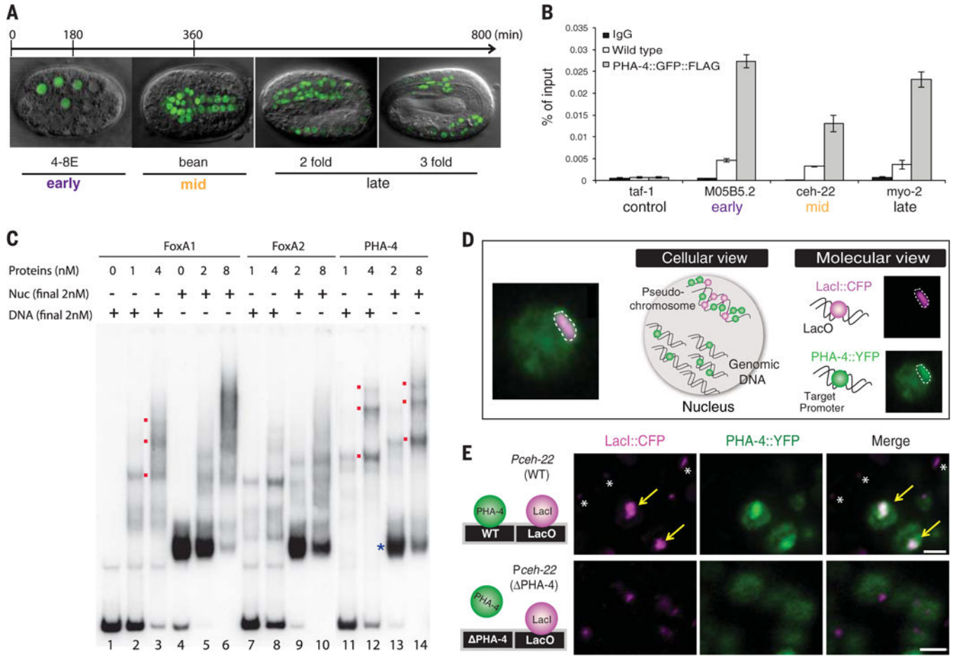
Fig. 1. PHA-4 is a pioneer factor
