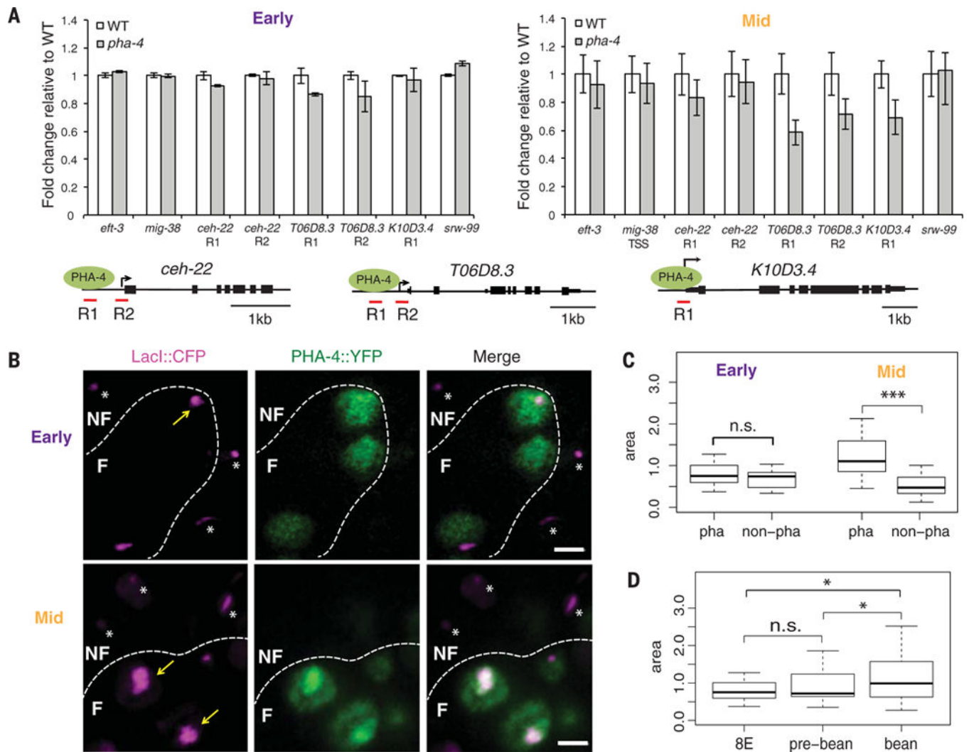
Fig. 4. PHA-4 promotes chromatin openness during mid-stage embryogenesis (A) Chromatin opening tracked by FAIRE–quantitative PCR. Early (left), FAIRE signals for three poised foregut genes were similar between wild-type (white) and pha-4(ts) (gray). Mid- (right), FAIRE signals were reduced at poised foregut genes in pha-4(ts) embryos. The gene structures show positions for PHA-4 binding (R1) and TSS (R2) sites. n = 3 replicates, mean \pm SEM. (B) Artificial chromosomes (CFP: :LacI, purple) bearing the ceh-22 promoter bound by PHA-4: :YFP (green) in early and mid-stage embryos. Dotted lines distinguish foregut (F) from nonforegut (NF). Scale bar, 2 \mu m. (C) Areas of artificial chromosomes carrying the ceh-22 promoter in foregut (pha) versus nonforegut (non-pha). (D) Areas of artificial chromosomes carrying the ceh-22 promoter in the foregut at different stages. * P = 0.01 to 0.05 ; *** P < 0.001 .
