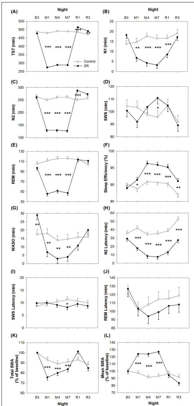
Figure 2 —Effects of sleep restriction on sleep macrostructure and SWA power across experimental nights. Mean \pm SEM of the SR (black filled circles) and the Control (gray open circles) groups were plotted for the last baseline night (B3), first, fourth, seventh sleep manipulation nights (M1, M4, and M7), and first and third recovery nights (R1 and R3). Asterisks indicate significant differences between groups for each night (* P < 0.05 , ** P < 0.01 , *** P < 0.001 ).
