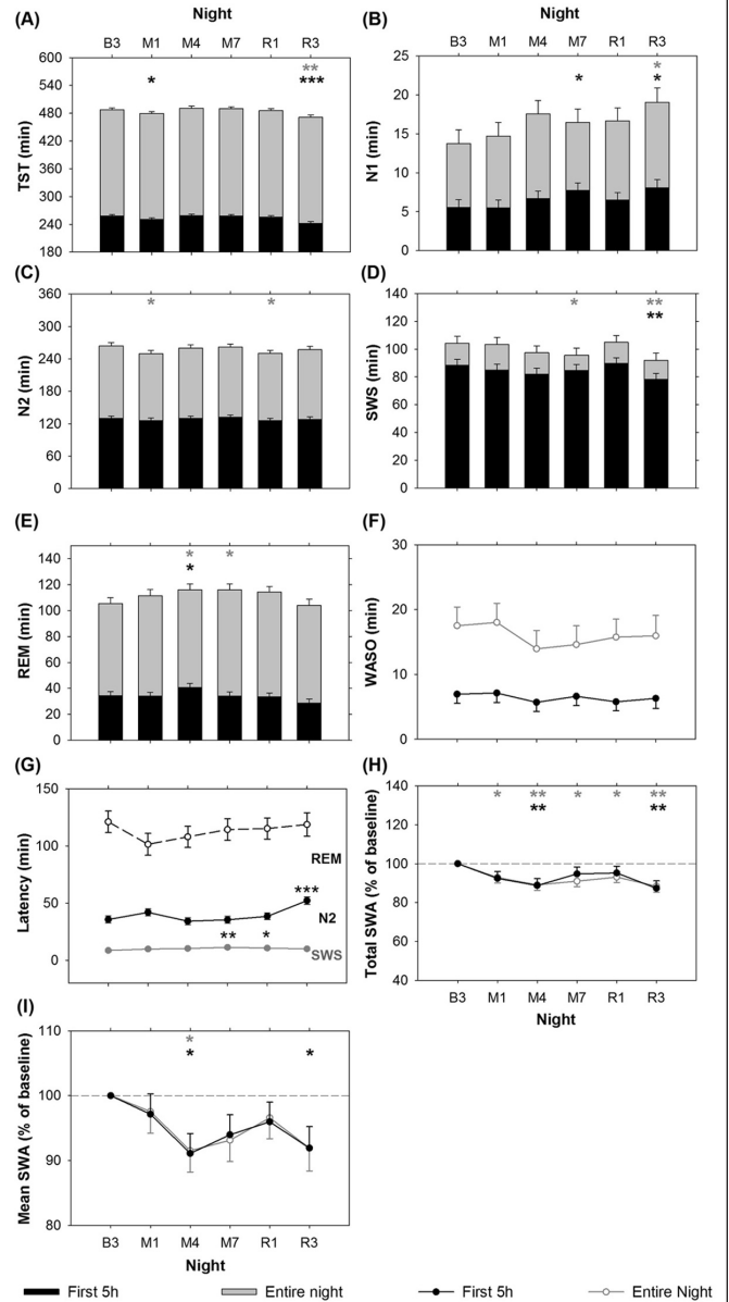
Figure 4 —Sleep macrostructure and SWA power of the Control group. Black bars indicate mean \pm SEM of sleep variables in the first 5 h of sleep for all nights, while gray bars indicate mean \pm SEM in the remainder of full sleep (9 h for B3, R1, and R3). Black asterisks indicate significant differences from B3 considering only the first 5 h of sleep while gray asterisks indicate differences from B3 considering the full sleep opportunity. (* P < 0.05 , ** P < 0.01 , *** P < 0.001 ).
