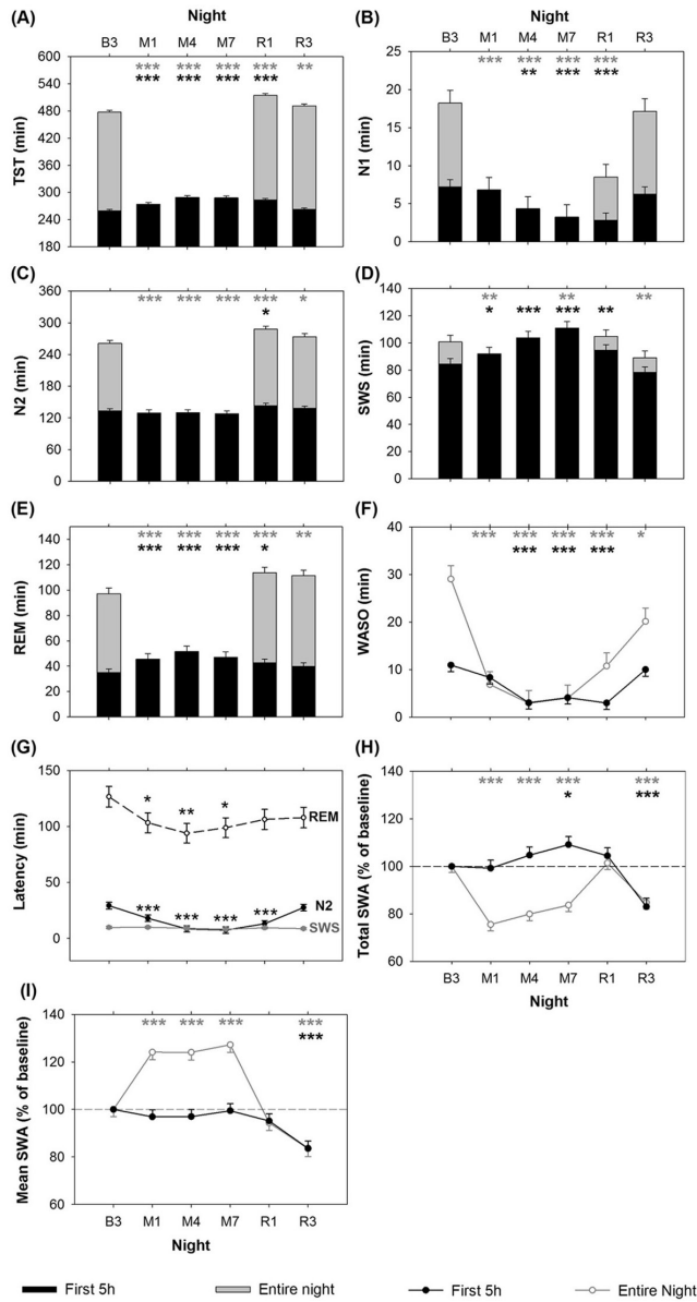
Figure 3 —Sleep macrostructure and SWA power of the SR group. Black bars indicate mean \pm SEM of sleep variables in the first 5 h of sleep for all nights, while gray bars indicate mean \pm SEM in the remainder of full sleep (9 h for B3, R1, and R3). Black asterisks indicate significant differences from B3 considering only the first 5 h of sleep in all nights while gray asterisks indicate differences from B3 considering the full sleep opportunity. (* P < 0.05 , ** P < 0.01 , *** P < 0.001 ).
