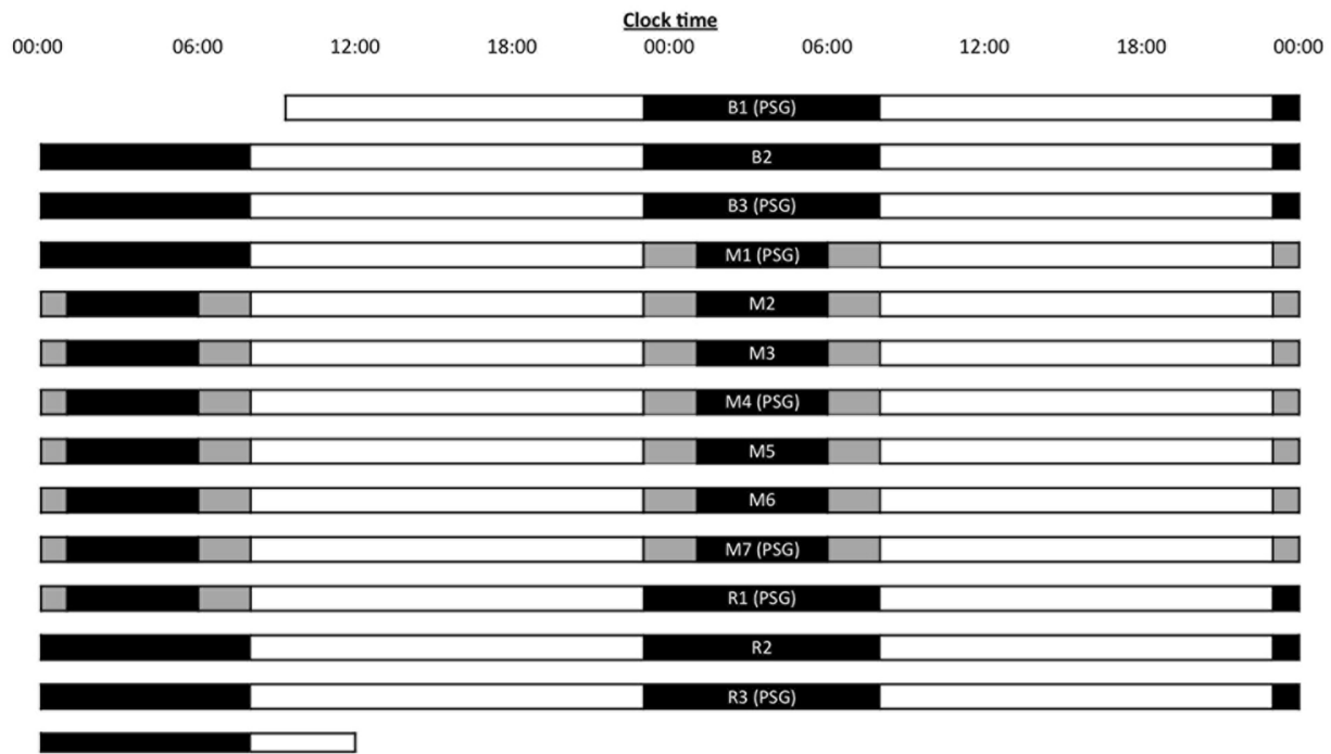
Figure 1 —Two-week experimental protocol illustrated in a double raster plot. Both SR and Control groups underwent 3 baseline nights of 9 h sleep opportunity (B1 to B3), followed by 7 nights of either 5 h (SR; black bars) or 9 h (Control; gray bars) sleep opportunity (M1 to M7), and ending with 3 recovery nights of 9 h sleep opportunity (R1 to R3). Nights where polysomnography (PSG) was recorded are indicated on the plot.
