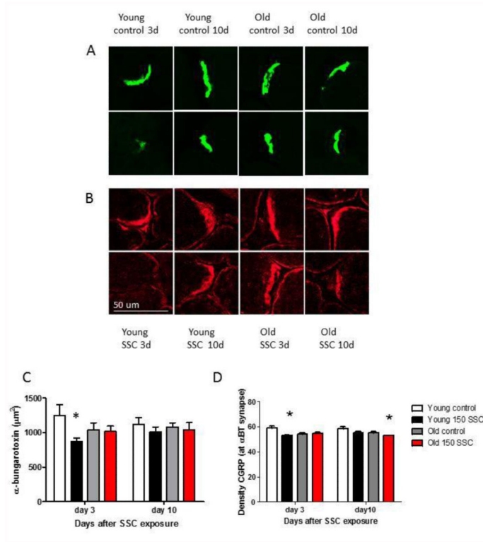
Figure 4. Photomicrographs showing \alpha BT staining (A) and CGRP staining (B) at the neuromuscular junction. The top row of each panel are photomicrographs from control rats and the bottom panels are photos from iSSC exposed rats. The area stained with \alpha BT in samples of the NMJ are presented in C. Young rats showed a reduction in the area stained with \alpha BT 3 days following iSSC exposure (* p < 0.05 , less than age-matched controls). There were no other significant changes in \alpha BT staining. The density of CGRP staining that was co-localized with \alpha BT and the NMJ is presented in Figure D. CGRP staining was reduced at the NMJ of young rats 3 days following iSSC exposure. By 10 days CGRP was back to control levels at the NMJ of young rats. However in old rats exposed to iSSCs, CGRP at the synapse was reduced (* p < 0.05 , less than age-matched controls, Bar in Figure B is 50 \mu m).
