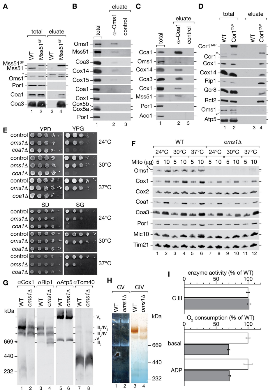
FIGURE 3: Loss of Oms1 effects mitochondrial supercomplexes. (A) WT and Mss51 SF mitochondria were solubilized in 1% digitonin buffer and complexes purified by StrepTactin Sepharose chromatography. After acidic elution, the eluate was analyzed by SDS-PAGE and Western blotting (total 1.5%, eluate 100%). Asterisks indicates unspecific antibody signal. Coimmunoprecipitation of Oms1 (B) or Coa1 (C) and control from digitonin-solubilized mitochondria. Eluates were analyzed by SDS-PAGE and Western blotting (total 1.5%, eluate 100%). (D) Mitochondria were solubilized with digitonin-containing buffer and supercomplexes isolated via TAP-tagged Cor1 using IgG chromatography followed by TEV protease cleavage. Eluates were analyzed as in B (total, 10%; eluate, 100%). Asterisks indicate cross-reaction of the antibodies. (E) Growth test on fermentable and nonfermentable full (YPD, YPG) and synthetic (SD –Trp, SG –Trp) media. WT, oms1Δ , and coa1Δ cells were spotted in serial 10-fold dilutions and incubated at indicated temperatures. (F) Steady-state protein level analysis of WT and oms1Δ mitochondria isolated from cells grown in YPG at different temperatures (24, 30, 37°C). Indicated amounts of mitochondria (Mito) were separated by SDS-PAGE, followed by Western blotting. Western blot analysis (G) and in-gel activity staining for cytochrome c oxidase and F 1 F 0 ATP-synthase (H) after BN-PAGE separation. Cells for mitochondrial preparation were grown on YPG at 30°C. (I) Top, enzymatic activity assay of cytochrome c reductase (CIII) in WT (white bars) and oms1Δ (gray bars) mitochondria ( n = 3 , \pm SEM). Bottom, oxygen consumption measurement of mitochondria from WT (white bars) and oms1Δ (gray bars). Isolated mitochondria were incubated with NADH (basal) and successively combined with ADP (phosphorylating respiration; state 3) in a high-resolution respirometry chamber ( n = 4 , \pm SEM).
