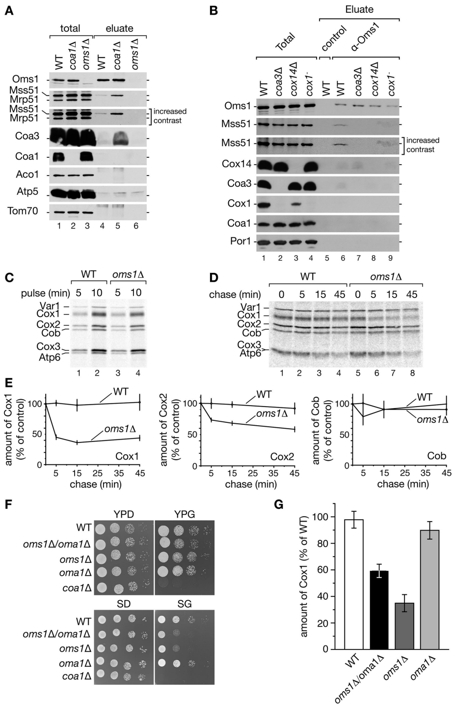
FIGURE 5: Oms1 acts in early steps of cytochrome c oxidase biogenesis. (A) Coimmunoprecipitation of Oms1 from digitonin-solubilized mitochondria isolated from WT, coa1Δ , and oms1Δ cells were analyzed by SDS-PAGE and Western blotting (total 1.5%, eluate 100%). (B) Immunoprecipitation of Oms1 as in A from WT, coa3Δ , cox14Δ , and cox1- mitochondria. Eluates were analyzed by SDS-PAGE and Western blotting (total 1%; eluate 100%). (C) In vivo pulse labeling of mitochondrial translation products using WT and oms1Δ cells. After [ 35 S] methionine labeling for 10 min at 30°C, whole-cell extracts were prepared and analyzed by SDS-PAGE and digital autoradiography. (D) Mitochondrial translation products were labeled with [ 35 S]methionine for 5 min as in C. Reactions were stopped by the addition of unlabeled methionine, and incubation continued at 30°C for the indicated chase times. Samples were processed as in C. (E) Signals of three independent experiments as shown in D were quantified using ImageQuant TL software. Bars represent the mean ratios of Cox1, Cox2, or Cob to Var1 relative to the signal after 0 min of chase (100%) for each individual strain ( n = 3, ±SEM). (F) Growth test on fermentable and nonfermentable full (YPD, YPG) and synthetic (SD, SG) media. (G) Quantification of in vivo labeling of mitochondrial translational products. Cells were labeled for 5 min and chased for 15 min. TCA-precipitated samples were separated by SDS-PAGE, quantified by digital autoradiography, and normalized for Var1 (C). n = 3; ± SEM.
