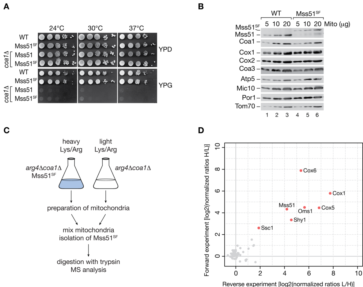
FIGURE 1: Oms1 interacts with Mss51. (A) Growth test on fermentable (YPD) and nonfermentable (YPG) full media. Cells were spotted in serial 10-fold dilutions and incubated at indicated temperatures. (B) Steady-state protein analysis from WT and Mss51-streptavidin-FLAG (Mss51 SF ) mitochondria. Indicated amounts of isolated mitochondria (Mito) were separated by SDS-PAGE, followed by Western blotting, and probed for indicated mitochondrial proteins. (C) Schematic illustration of Mss51 SF isolation for SILAC and mass spectrometry analysis. Representation of the forward experiment. For the reverse experiment, arg4Δcoa1Δ/Mss51 SF was grown on light medium and arg4Δcoa1Δ on heavy medium. (D) Scatterplot representation of normalized heavy/light (forward experiment) and light/heavy (reverse experiment) SILAC ratios after isolation of Mss51 SF (via StrepTactin Sepharose) from arg4Δcoa1Δ . Enriched proteins are displayed as red dots and other proteins in gray. The full list of identified proteins is given in Supplemental Table S1.
