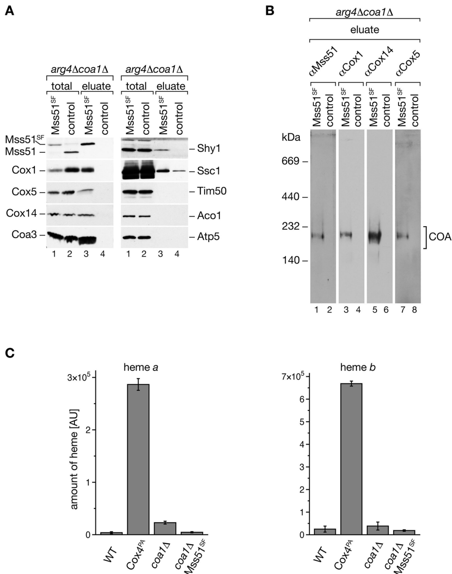
FIGURE 2: Characterization of the COA 220 complex in cells lacking Coa1. (A) Results of the SILAC analysis were confirmed by native purification of Mss51 SF -containing complexes. Eluates were separated by SDS-PAGE, followed by Western blot analysis. Amount of total sample loaded corresponds to 3% of the eluate. (B) Native eluted proteins (as in A) from coa1Δ/arg4Δ/Mss51 SF mitochondria were analyzed by BN-PAGE and Western blotting. As a control, the purification was performed from solubilized coa1Δarg4Δ mitochondria. (C) HPLC analysis of heme a and heme b in isolated mature cytochrome c oxidase and COA complexes. Heme a and heme b were extracted and quantified from eluates of native isolated Cox4 ProtA or Mss51 SF complexes ( n = 3 , \pm SEM).
