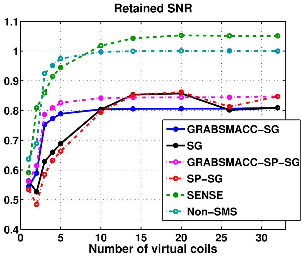
Figure 7. Average retained SNR, or equivalently, average 1/g -factor within brain voxels.
