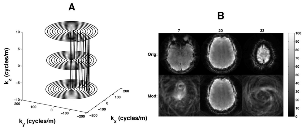
Figure 2. (a) Three-dimensional concentric ring k -space trajectory. (b) Modulation pattern resulting from a blipped concentric ring trajectory for 3 simultaneous slices. The numbers at the top indicate the slice number, where contiguous slices in the volume are numbered 1 through 39. The 20th slice is acquired at z -isocenter, assuming an axial acquisition. The top row shows the original, non-modulated, 3 simultaneous slices. The bottom row shows what the blipped modulation does to the various slices. Slice 20 is unaffected because it is acquired at z -isocenter. The blipped-EPI equivalent of slices 7 and 33 would be a simple FOV shift.
