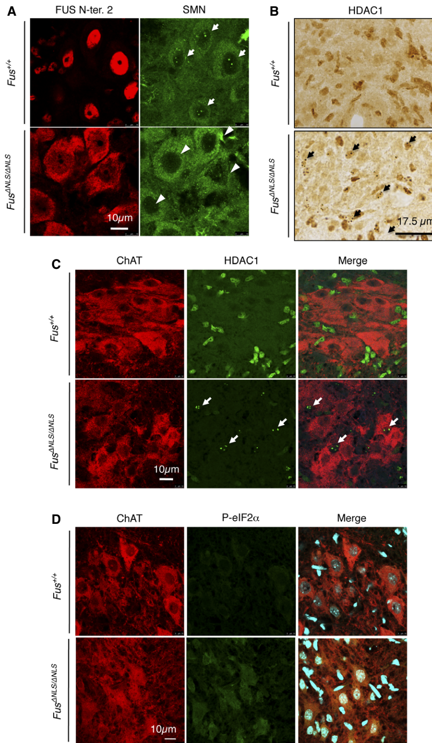
Figure 8. Alterations of SMN, HDAC1, and eIF2α in Fus ANLS/ANLS mice.
