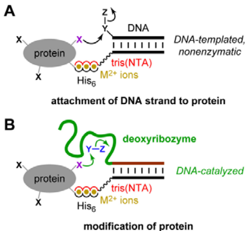
Fig. 1. Use of histidine tags to recruit reagents or catalysts for peptide and protein modification. (A) The reported use of hexahistidine (His 6 ) tags and divalent metal ions ( M^{2+} ) for directing nonenzymatic, DNA-templated reaction of protein side chains. 8 In one case, the authors instead used a natively metal-binding protein. NTA = nitrilotriacetic acid. (B) As evaluated in this study, the potential use of His 6 tags and M^{2+} to recruit a deoxyribozyme for catalyzing peptide and protein modification. See Fig. 2 for details of DNA catalysis arrangement, including reaction partner for the protein (shown here as Y–Z), as well as NTA structure.
