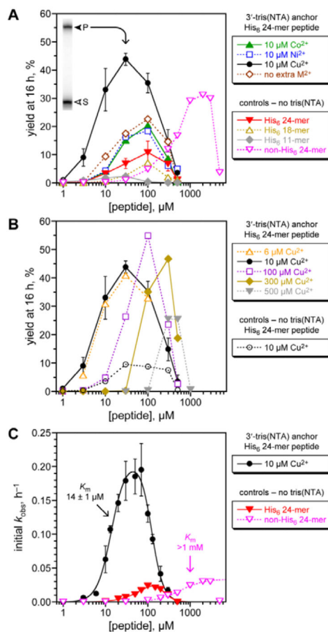
Fig. 3. Assessing histidine tag recruiting for the 8XJ105 deoxyribozyme. See the Experimental section for explanation of error bars in all panels. Conditions: 20 nM 3'- 32 P-radiolabeled 5'-pppRNA, 0.5 μM 8XJ105 deoxyribozyme, 2 μM 3'-tris(NTA) DNA anchor oligonucleotide, 1–5000 μM peptide, 70 mM HEPES, pH 7.5, 40 mM MgCl 2 , 20 mM MnCl 2 , 1 mM ZnCl 2 , 150 mM NaCl, and CoCl 2 , NiCl 2 , or Cu(NO 3 ) 2 as indicated at room temperature. CuCl 2 gave equivalent outcome. (A) Yield at 16 h of peptide-RNA conjugate as a function of concentration of His 6 -tagged 24-mer peptide (or untagged 24-mer in one case). All experiments including the controls were performed with 1 mM Zn 2+ ; 10 μM Co 2+ , Ni 2+ , or Cu 2+ was additionally present where indicated. Inset : PAGE data at 16 h for 3'- 32 P-radiolabeled RNA and 30 μM His 6 -tagged 24-mer peptide with Cu 2+ (S = substrate, P = product). See Fig. S1 (ESI † ) for data with 5'-tris(NTA) moiety. 24-mer H 6 SAGERASAEDMARAAYAA (for non-His 6 , replace H 6 with ASAASA); 18-mer H 6 SAEDMARAAYAA; 11-mer H 6 AAYAA. (B) Optimization of Cu 2+ concentration, and demonstration that Cu 2+ alone [without tris(NTA)] is not responsible for the recruiting effect. (C) Determination of peptide K_m values using initial-rate kinetics. See curve fit descriptions and fit details in the Experimental section.
