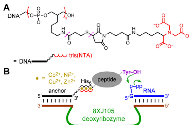
Fig. 2. Strategy for using histidine tags to recruit a deoxyribozyme to a peptide substrate and enable DNA-catalyzed peptide modification. (A) Tris(NTA)-modified DNA anchor oligonucleotide. The 3'-tris(NTA) moiety was connected to the DNA by a hexa(ethylene glycol) spacer. For the 5'-tris(NTA)-modified DNA anchor, the 5'-tris(NTA) moiety was connected to the DNA by a T 15 oligonucleotide spacer. Each tris(NTA)-modified oligonucleotide was synthesized by a multistep procedure in which the linkages marked with dashes were created (see the Experimental section). (B) Design showing the intended interactions among the 8XJ105 deoxyribozyme that forms nucleopeptide linkages, 3'-tris(NTA)-modified DNA anchor, His 6 -tagged peptide substrate, and divalent metal ions. Success is revealed by either or both of increase in peptide-RNA conjugation yield and leftward shift in peptide concentration dependence.
